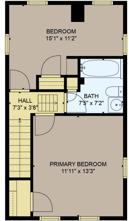
FLOOR 3
