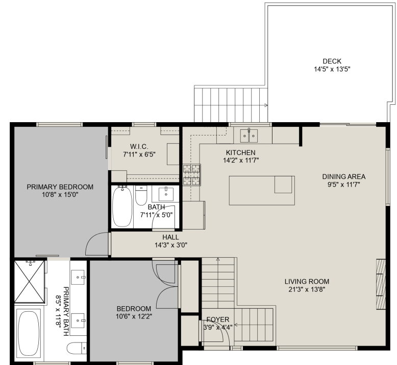
FLOOR 2
