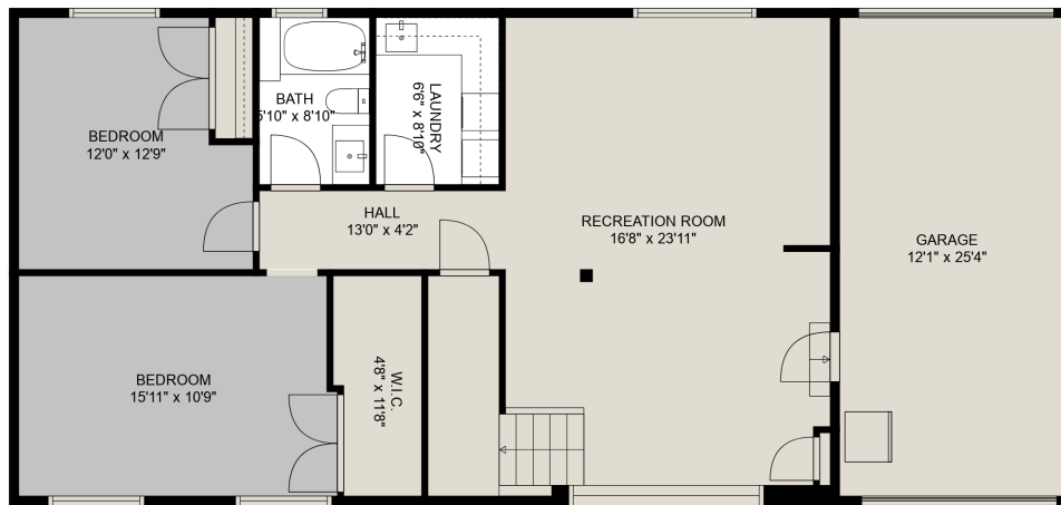
FLOOR 1
