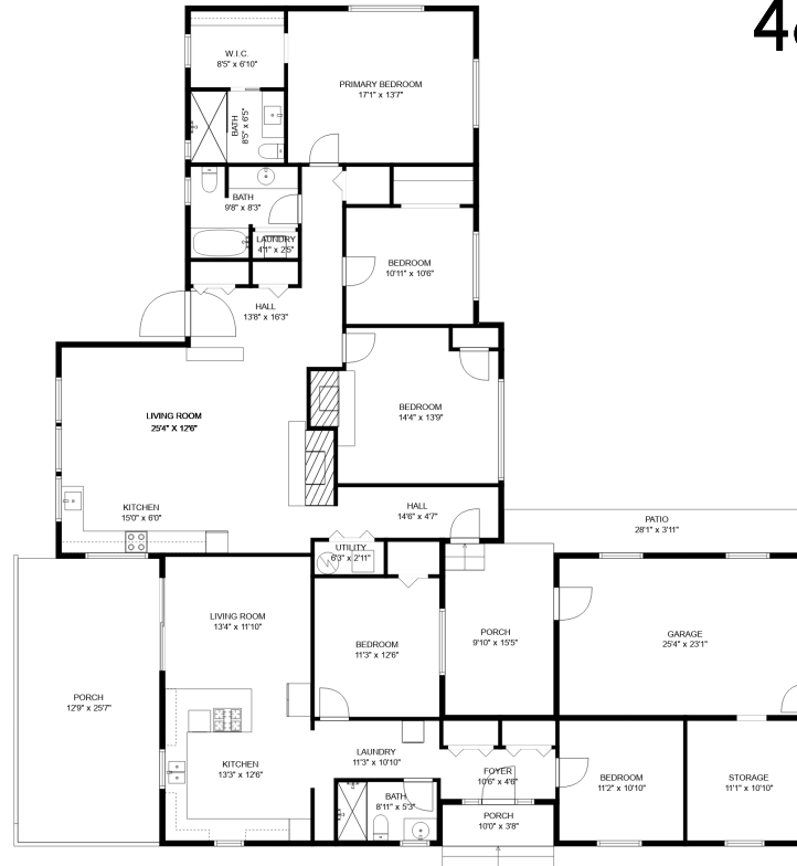
FLOOR 2
