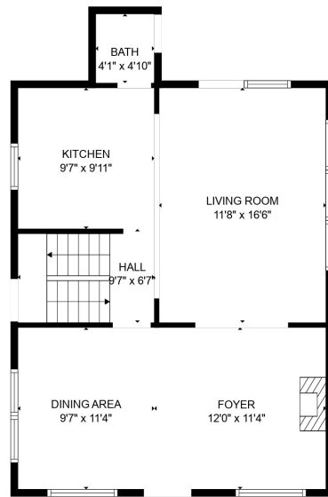
FLOOR 2
