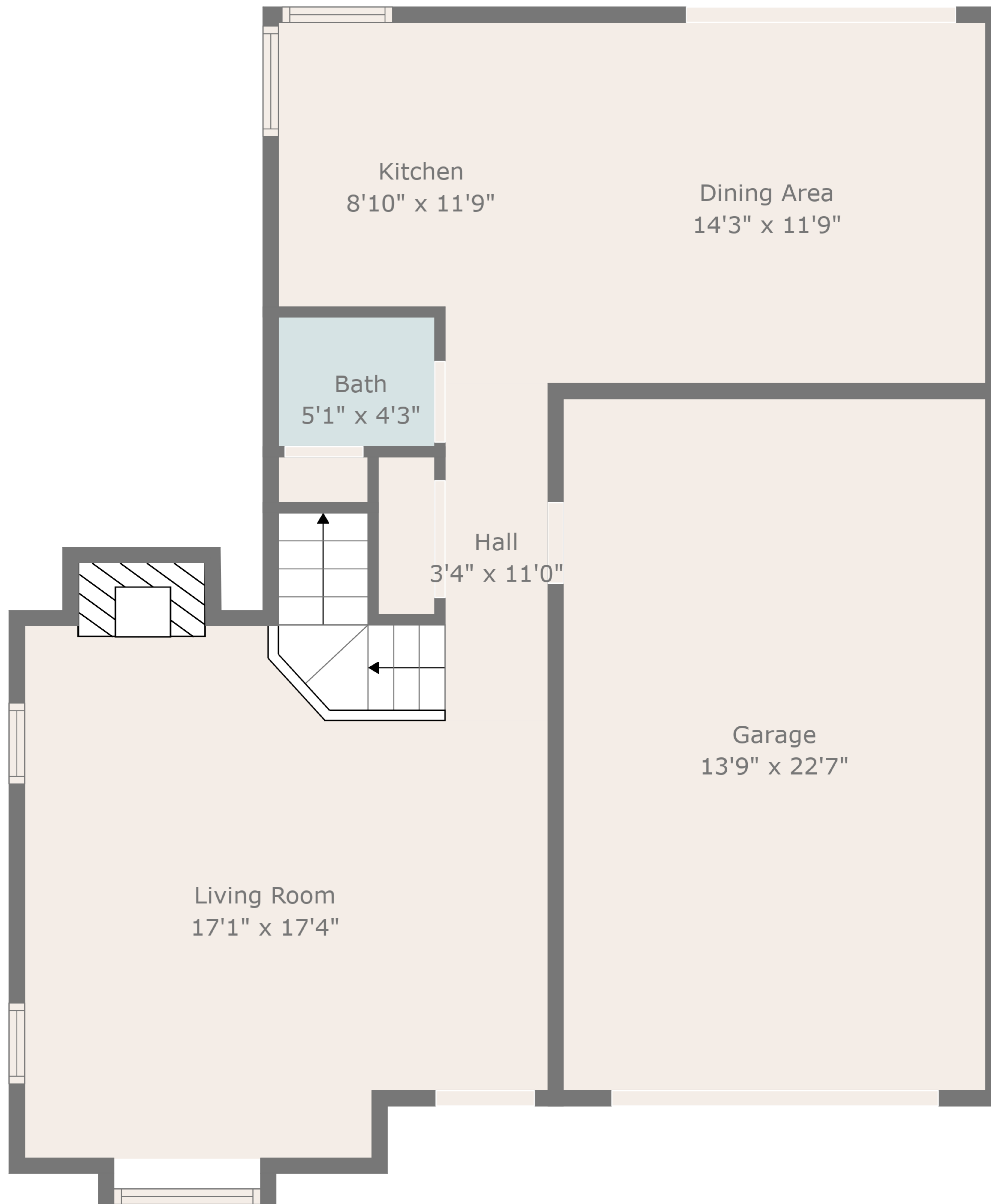
Floor 1
