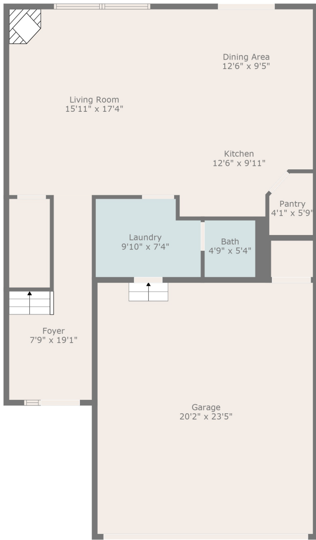
Floor 1
