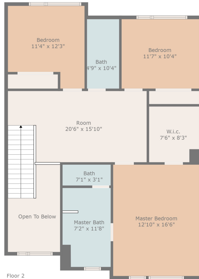
Floor 2
