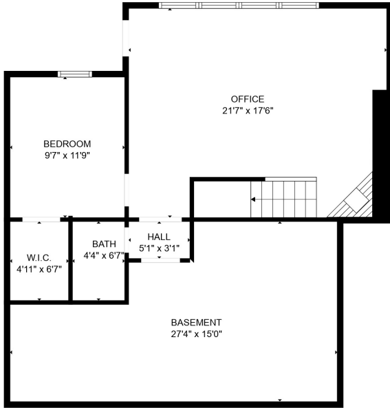
FLOOR 1
