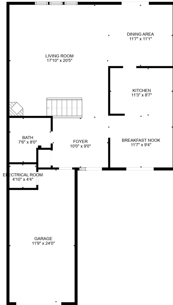
FLOOR 1
