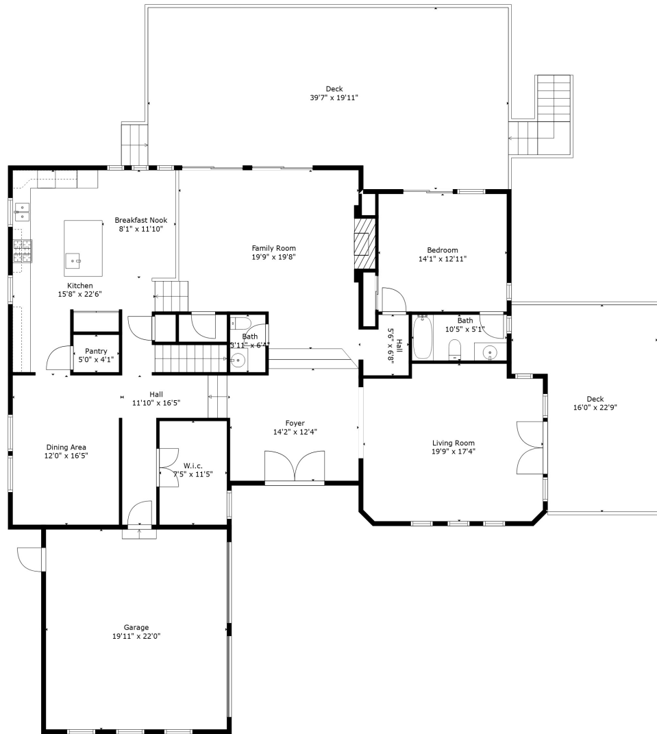
Floor 1
