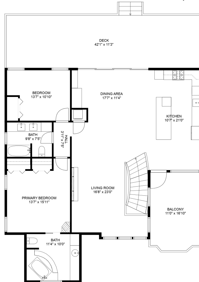
FLOOR 2
