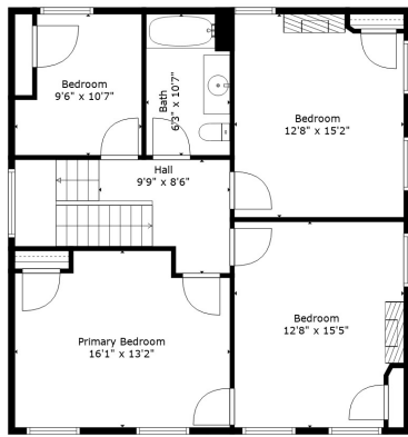
Floor 3
