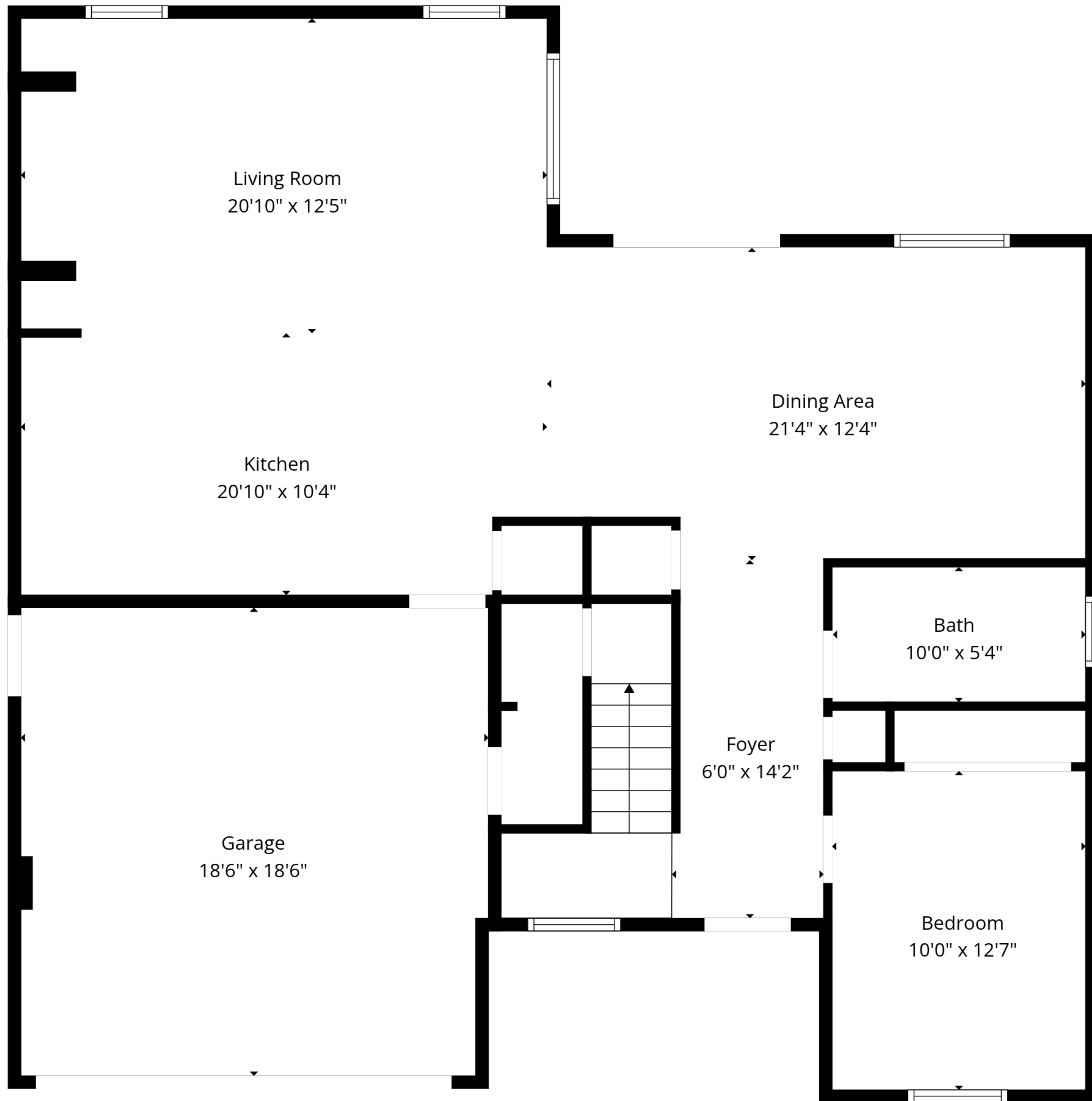
1st Floor
