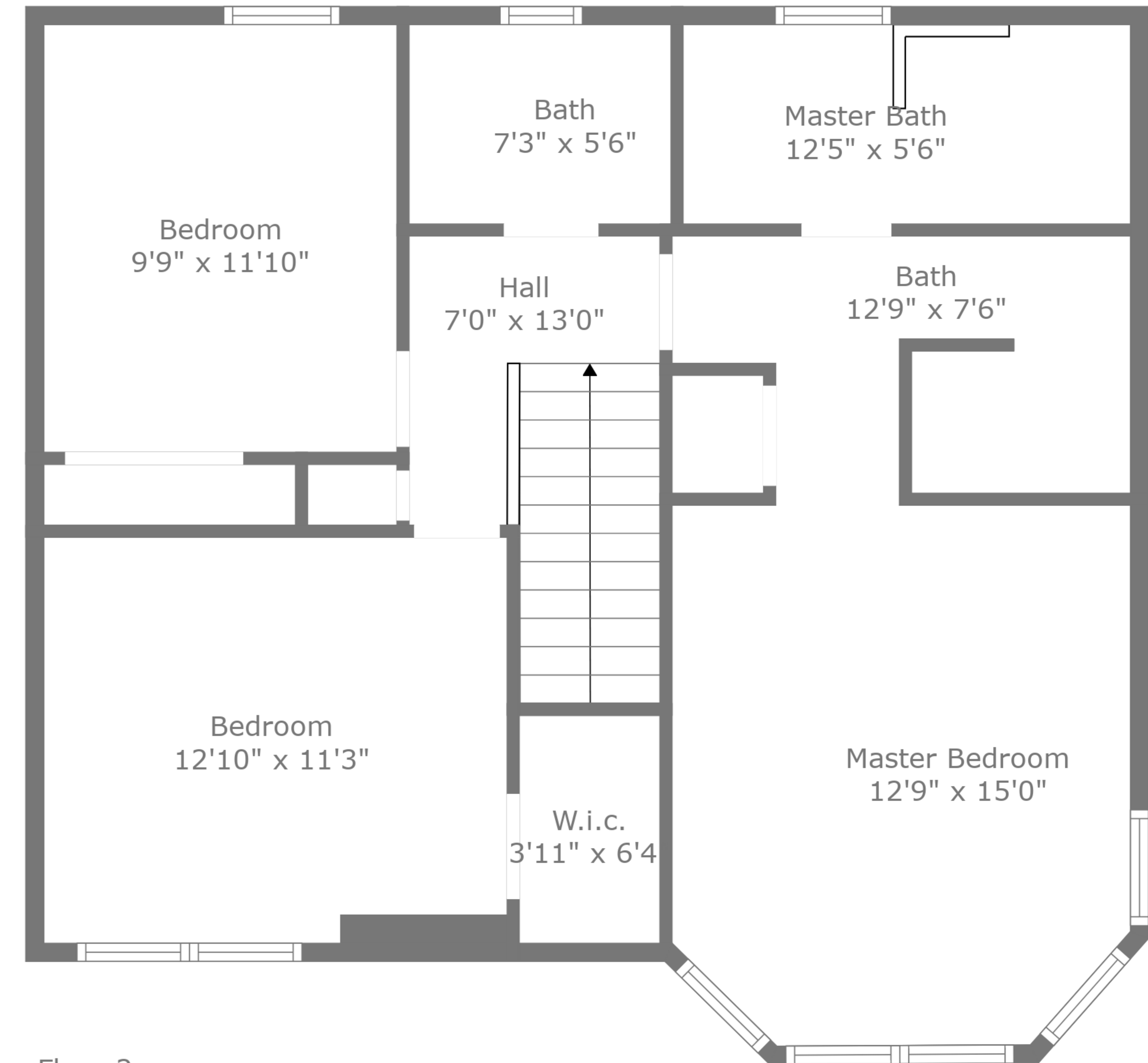
Floor 2
