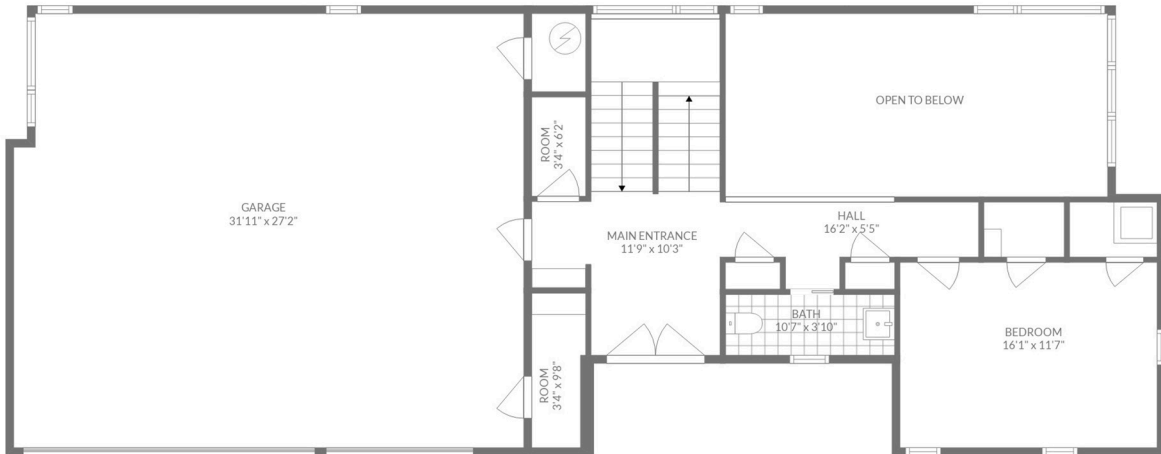
FLOOR 2
