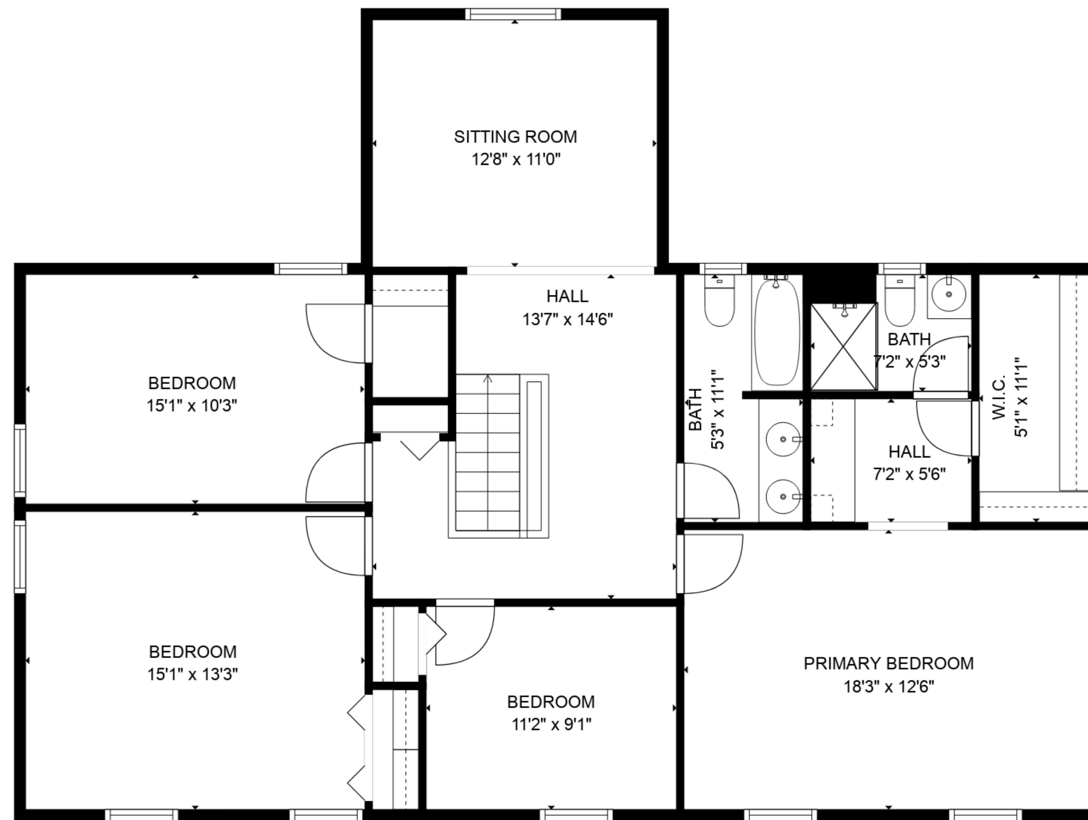
FLOOR 3
