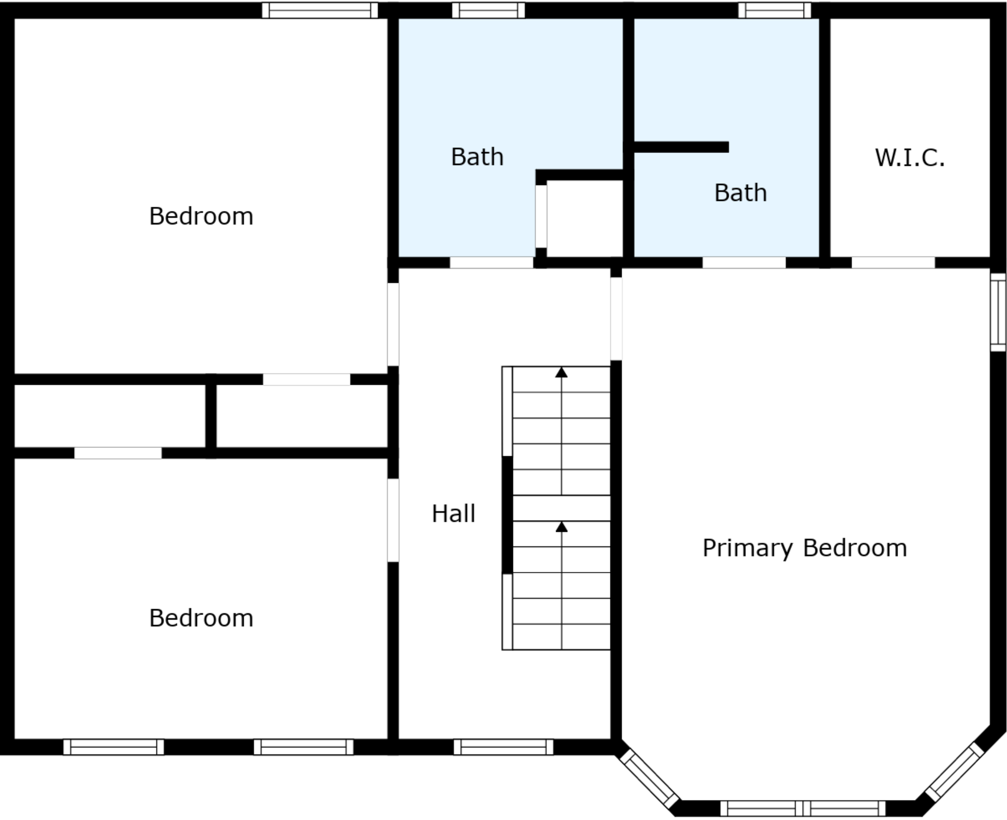
Floor 2
