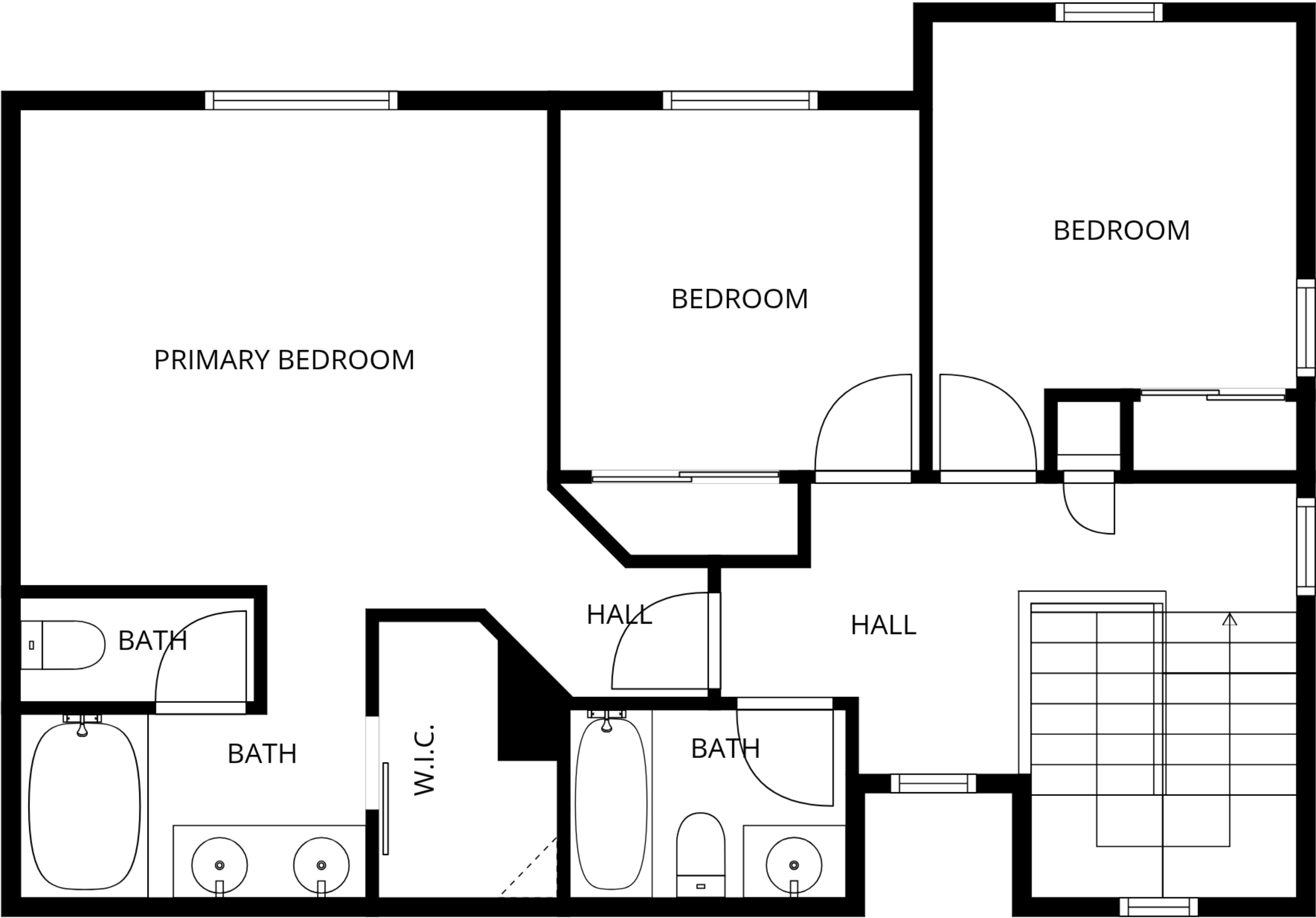
FLOOR 2
