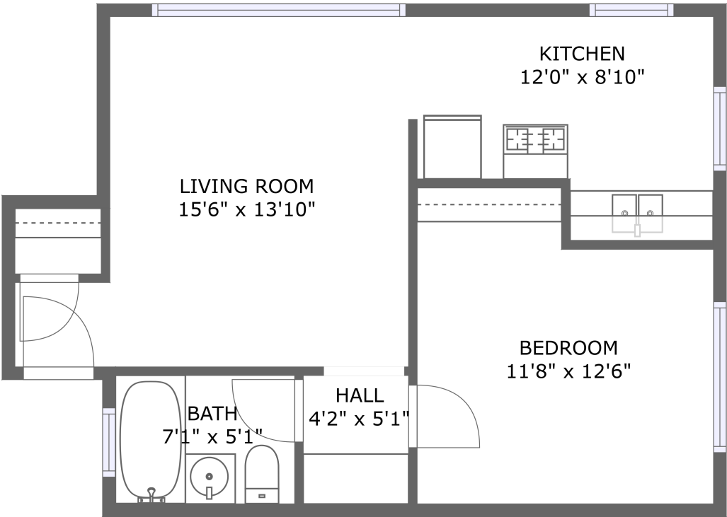
FLOOR 1
