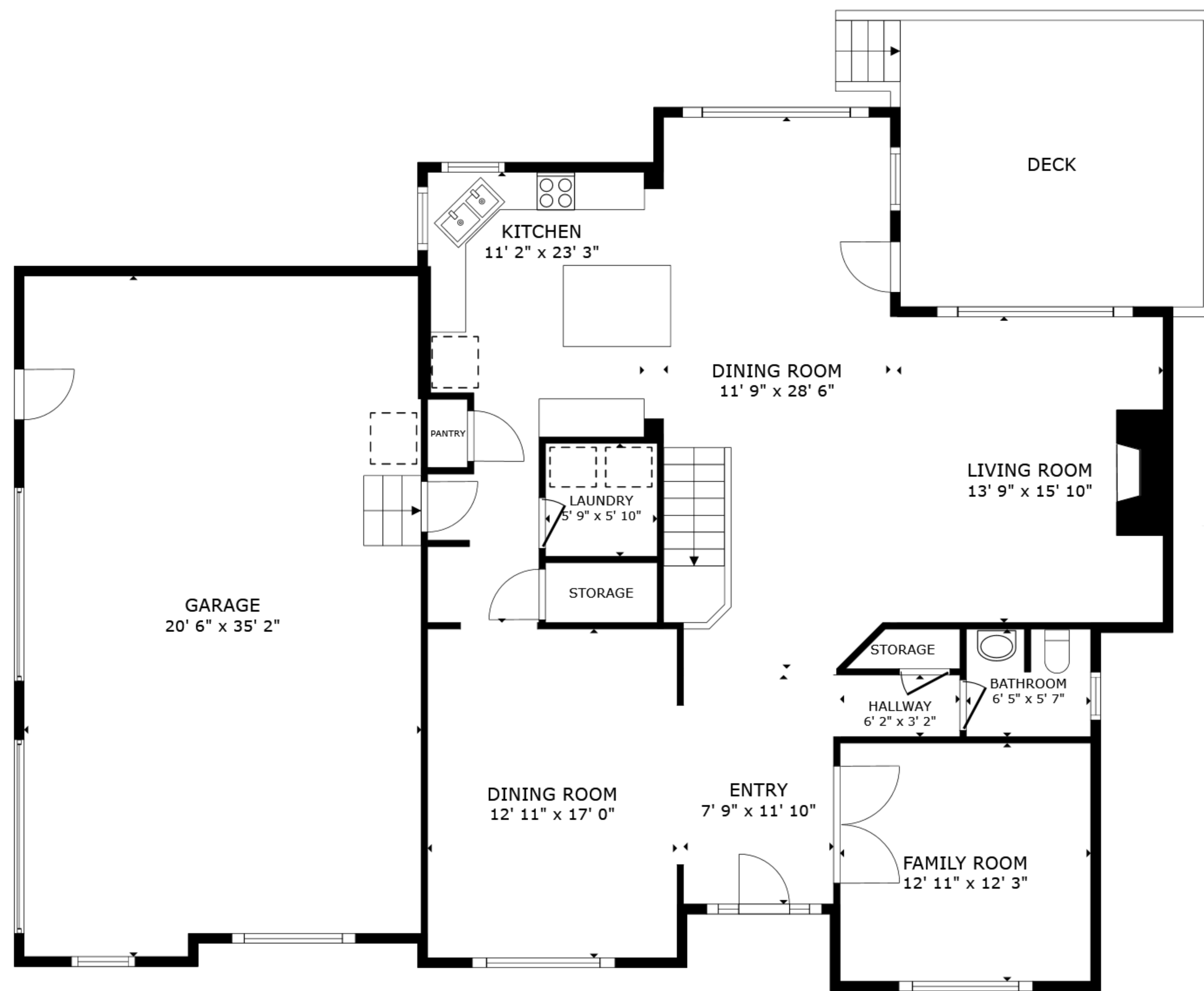
FLOOR 1
