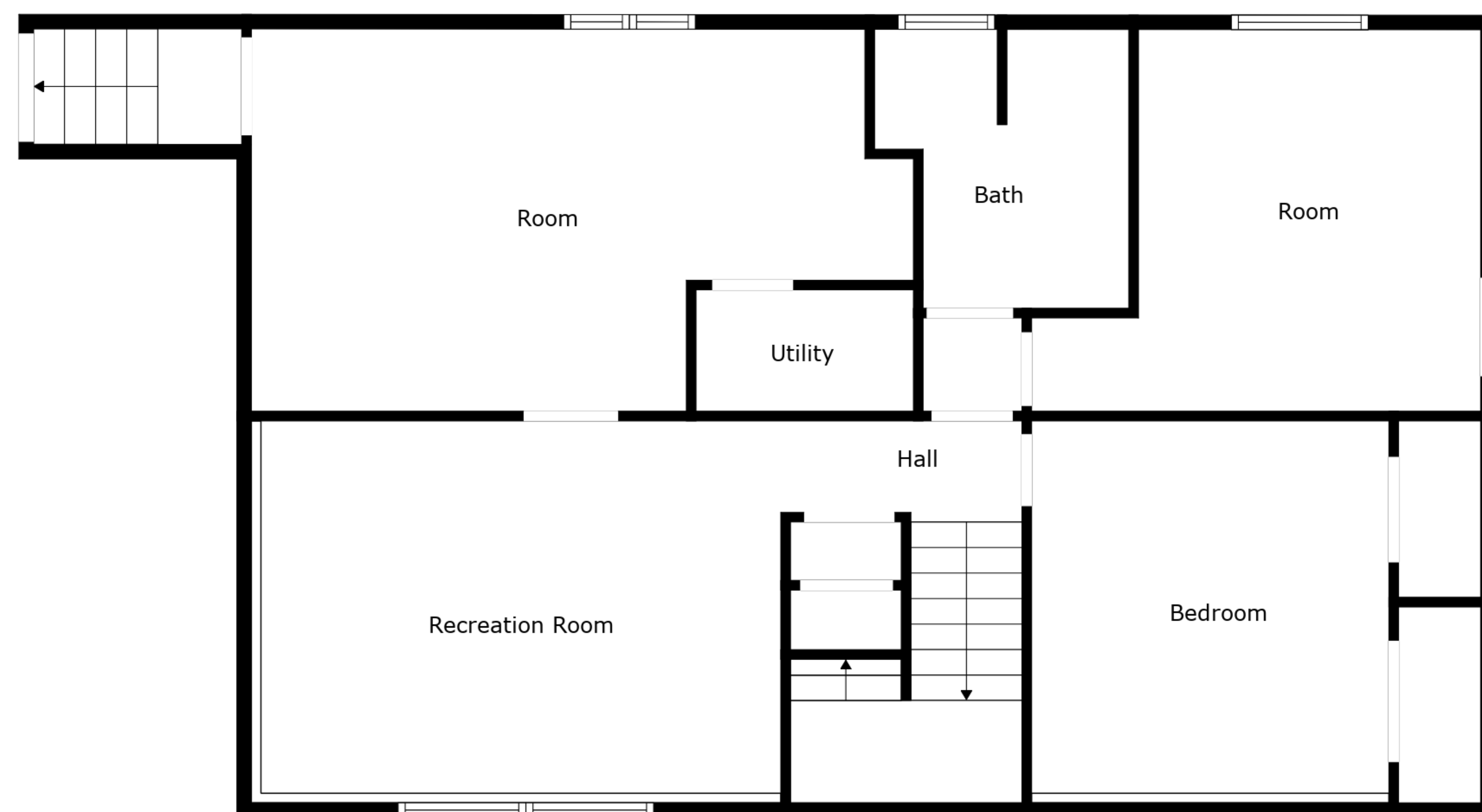
Floor 1
