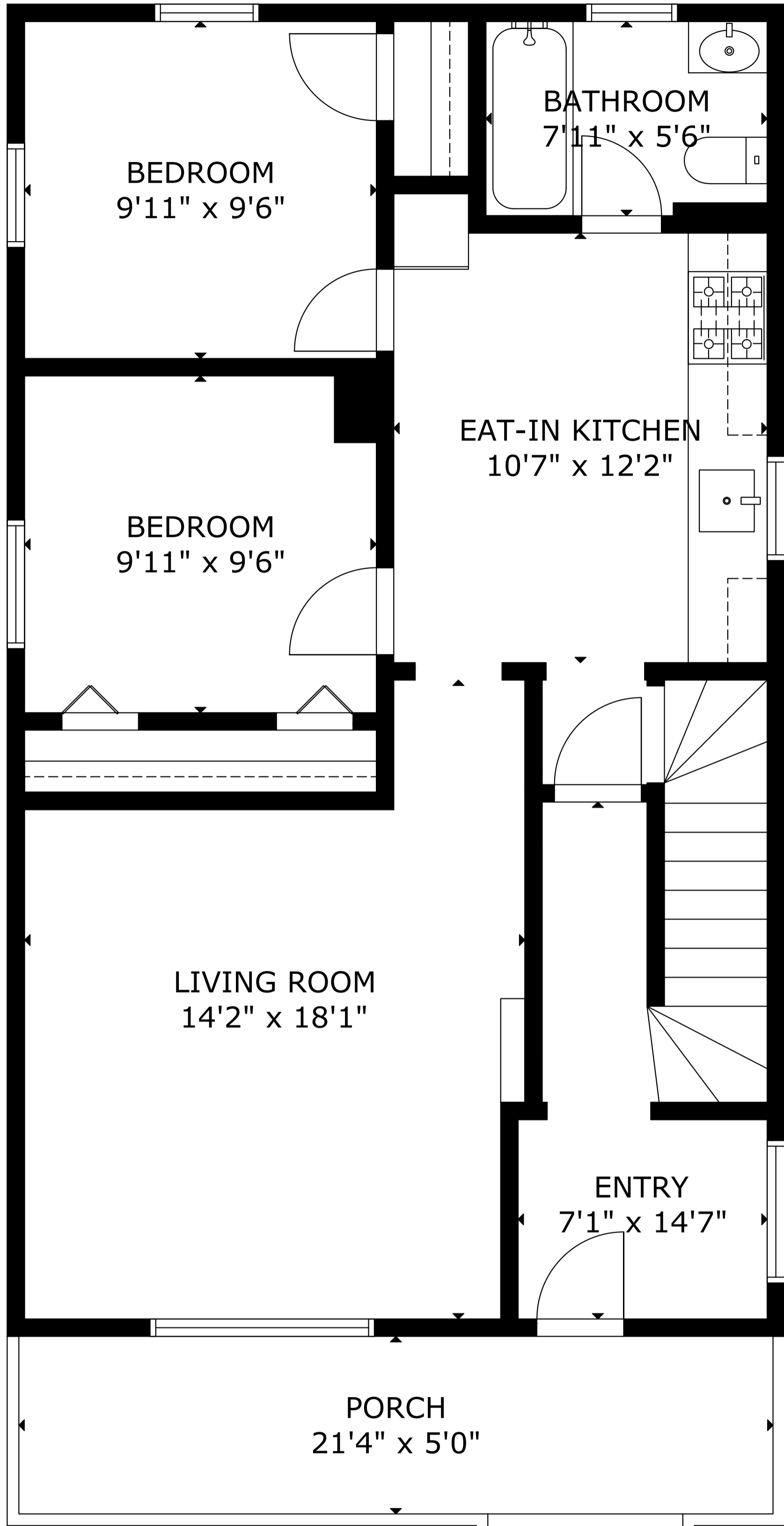
FIRST FLOOR
