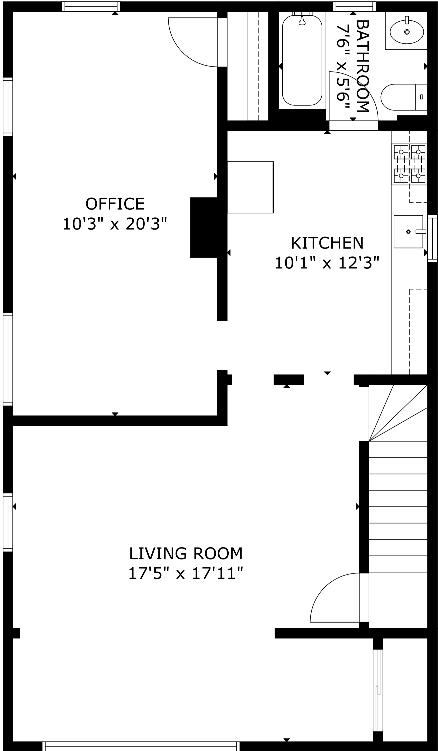
SECOND FLOOR
