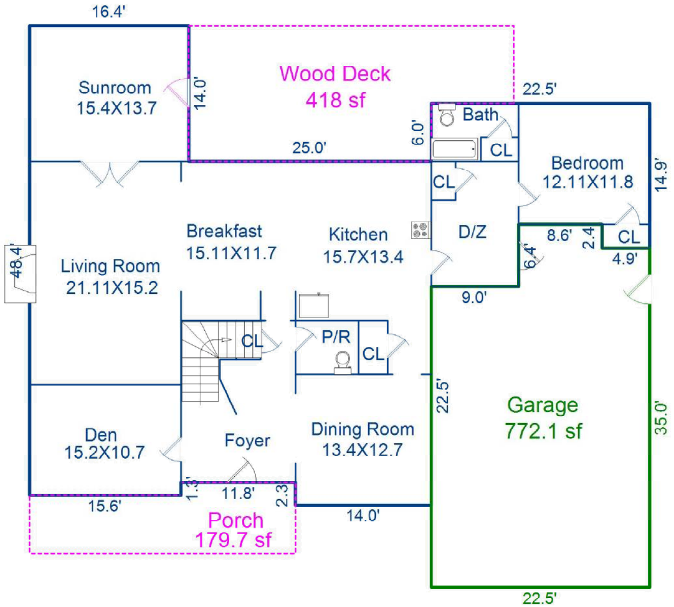
First Floor 2003 sf
