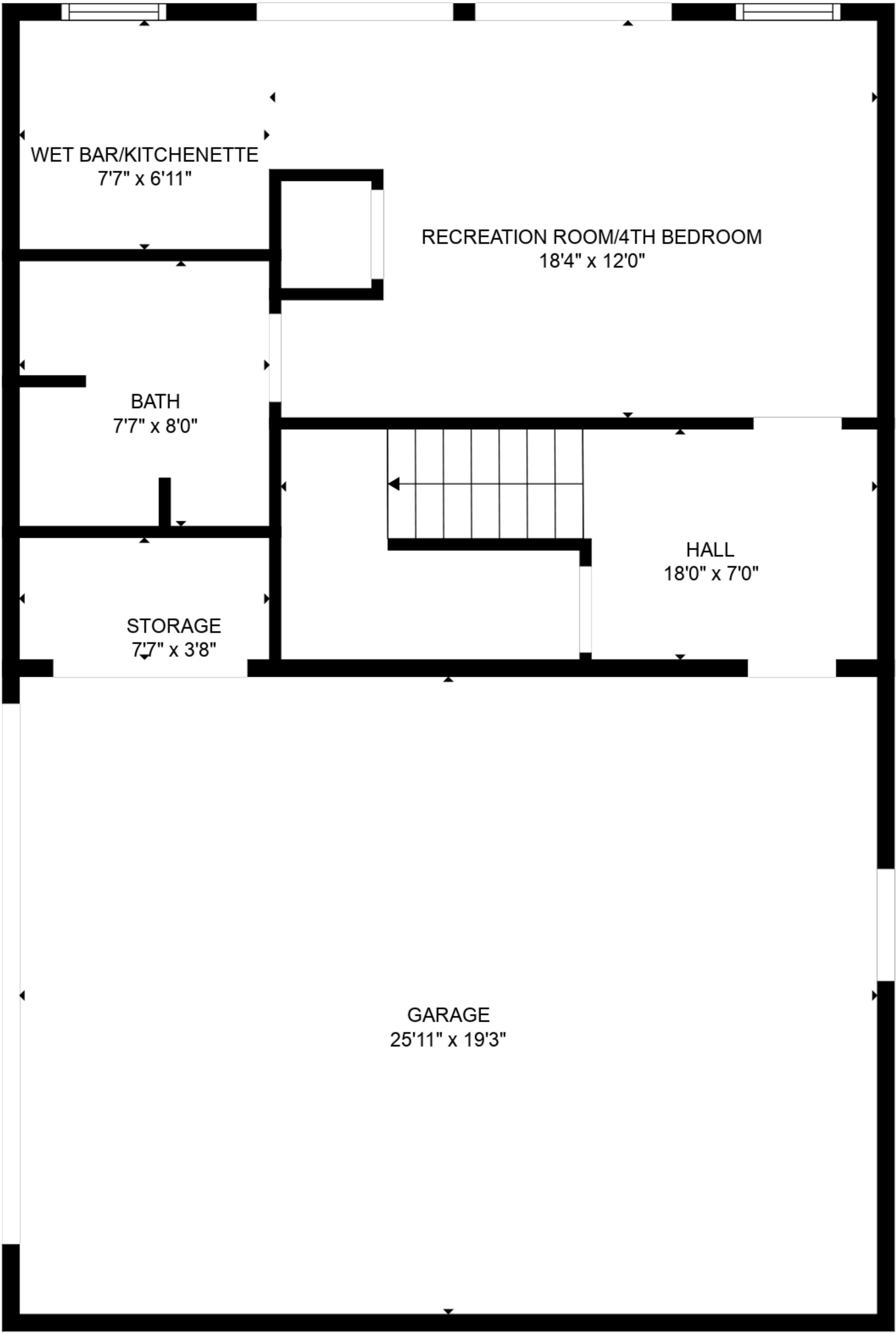
FLOOR 1
