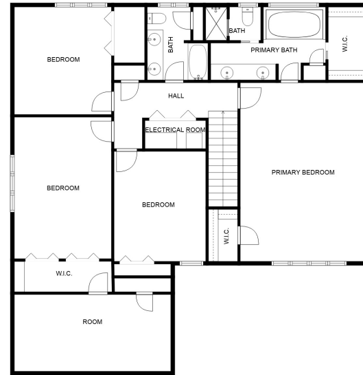
FLOOR 3
