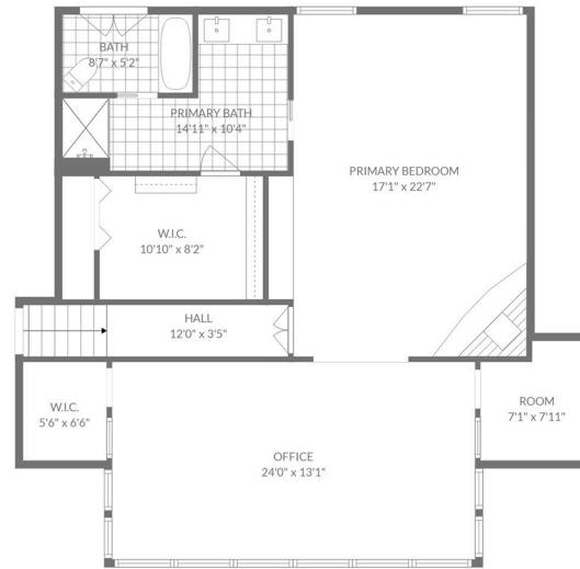
FLOOR 2
