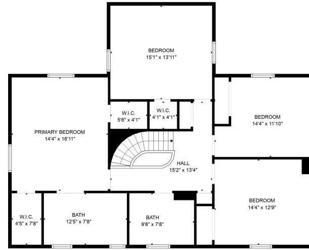
FLOOR 3
