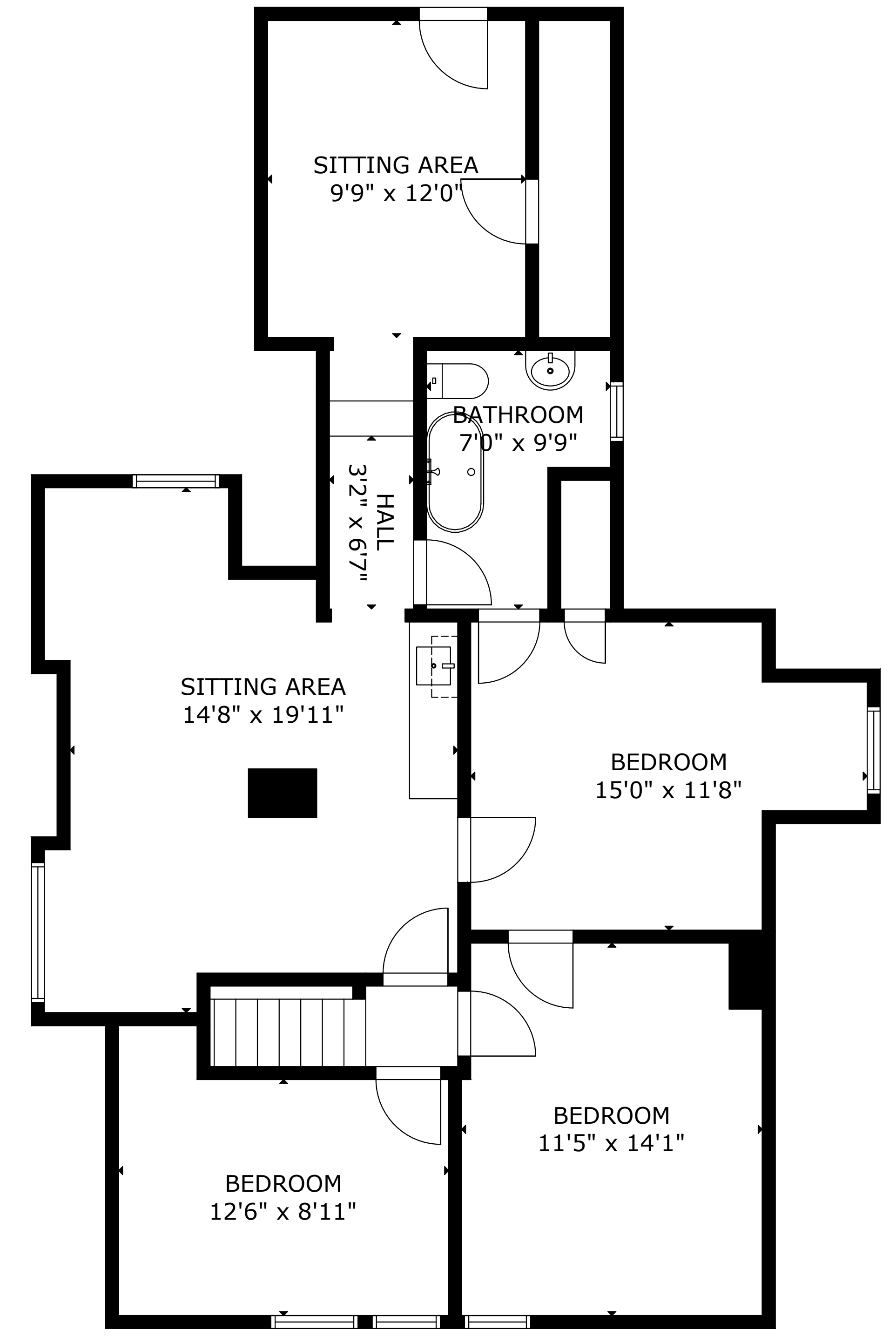
UPPER LEVEL 2
