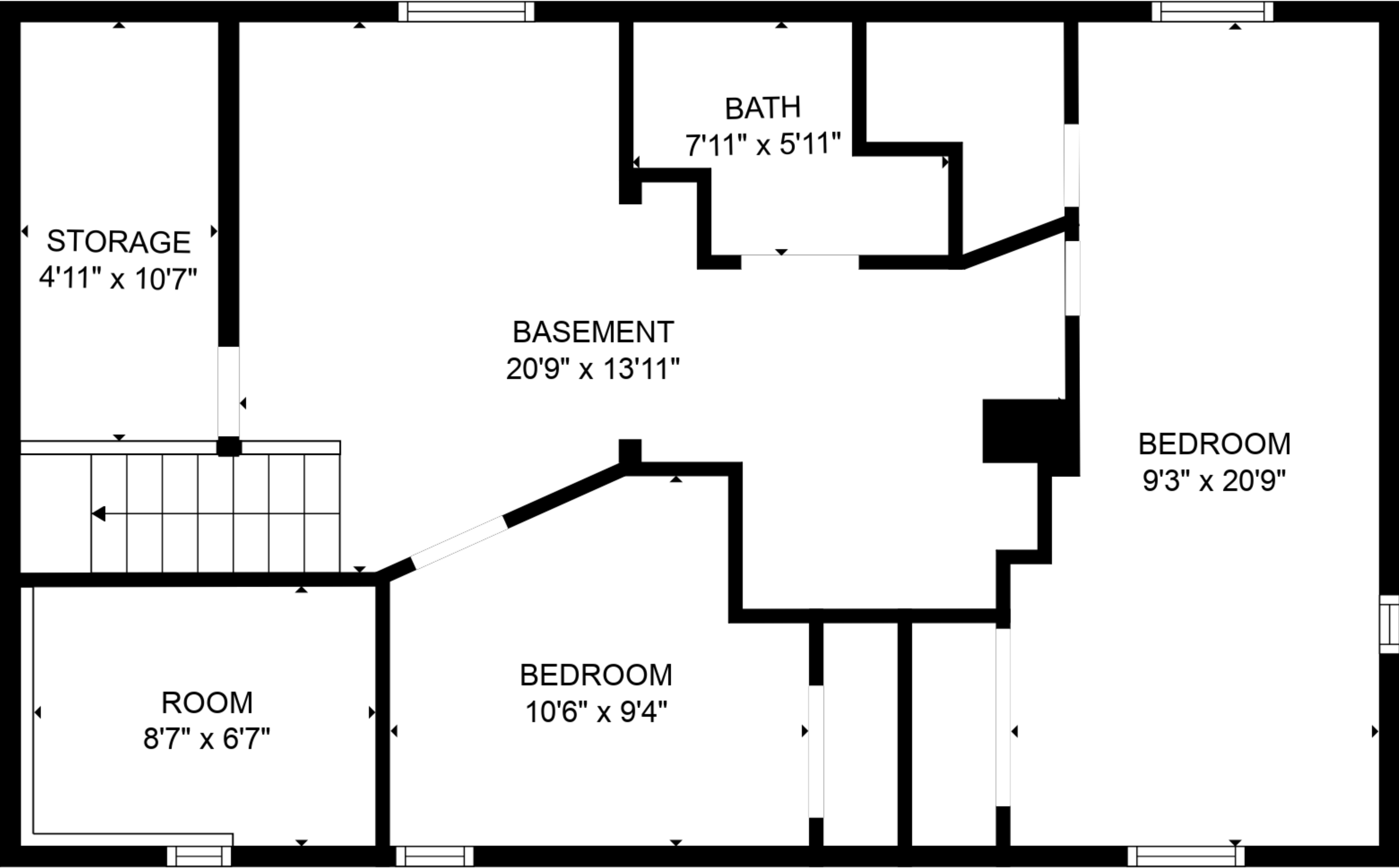
FLOOR 1
