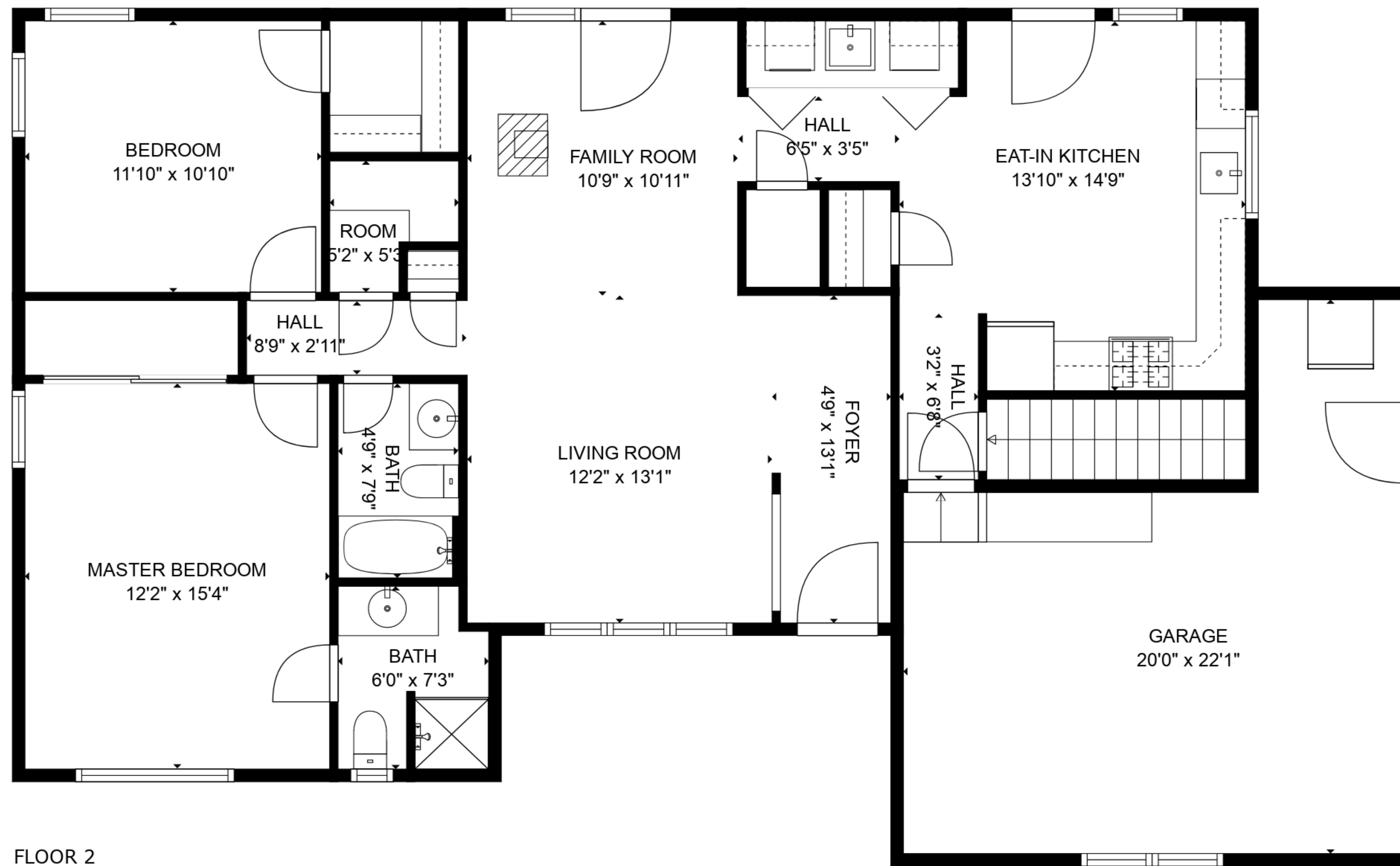
FLOOR 2
