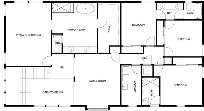
FLOOR 3
