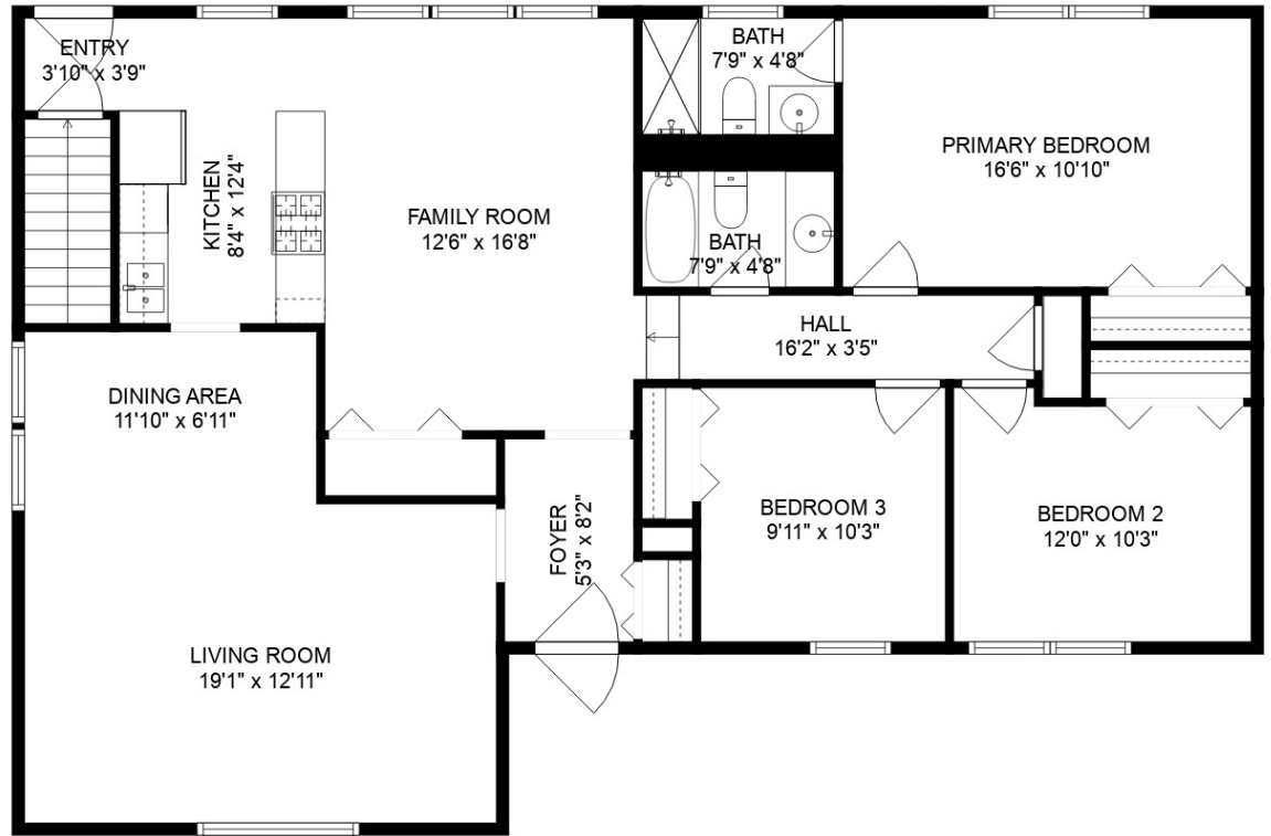
MAIN FLOOR
