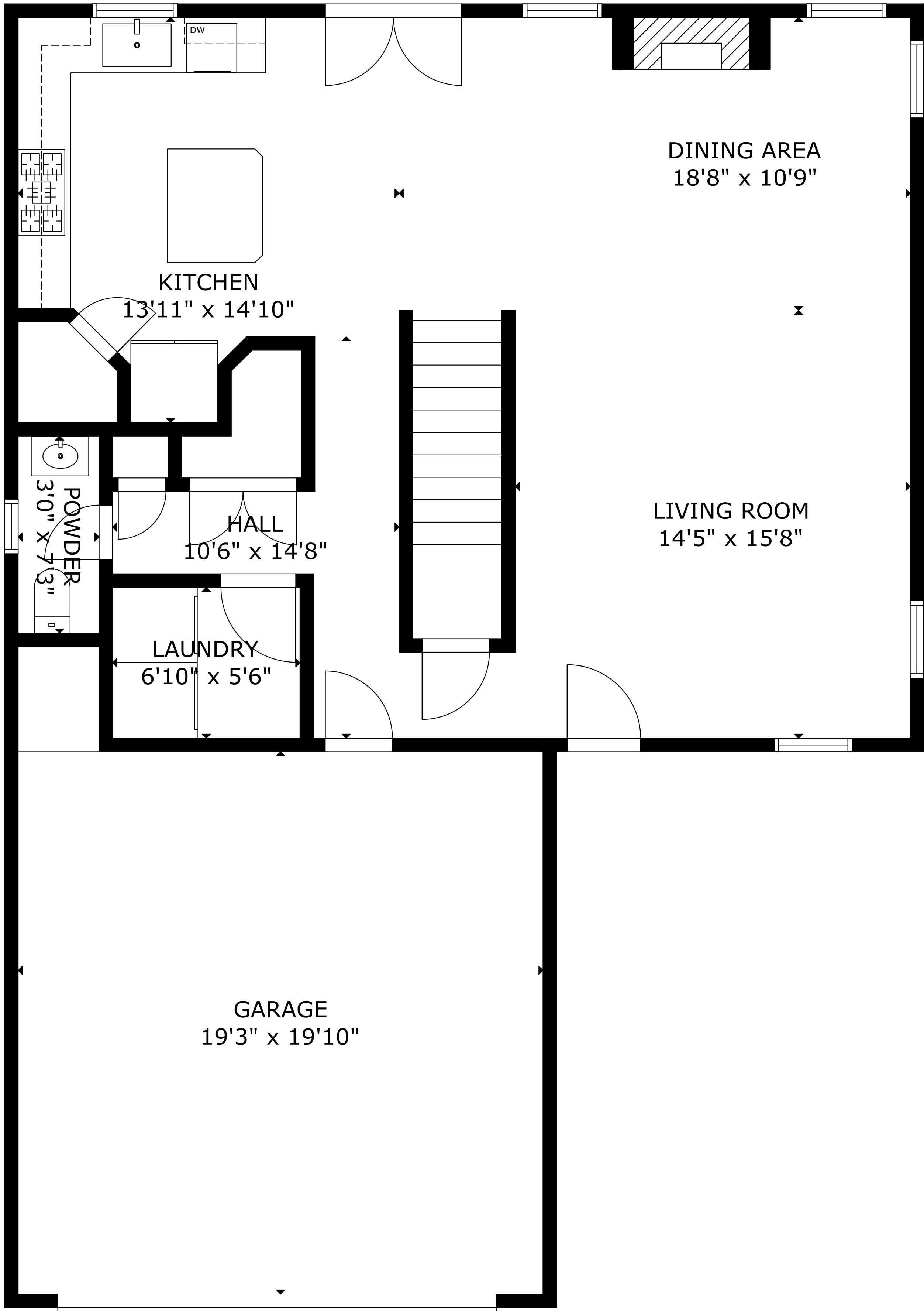
FLOOR 1
