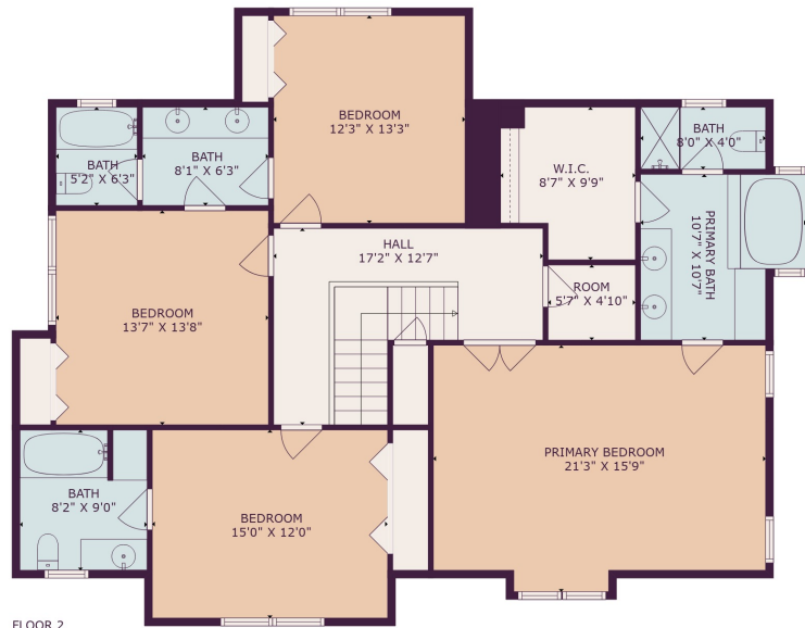
FLOOR 2
