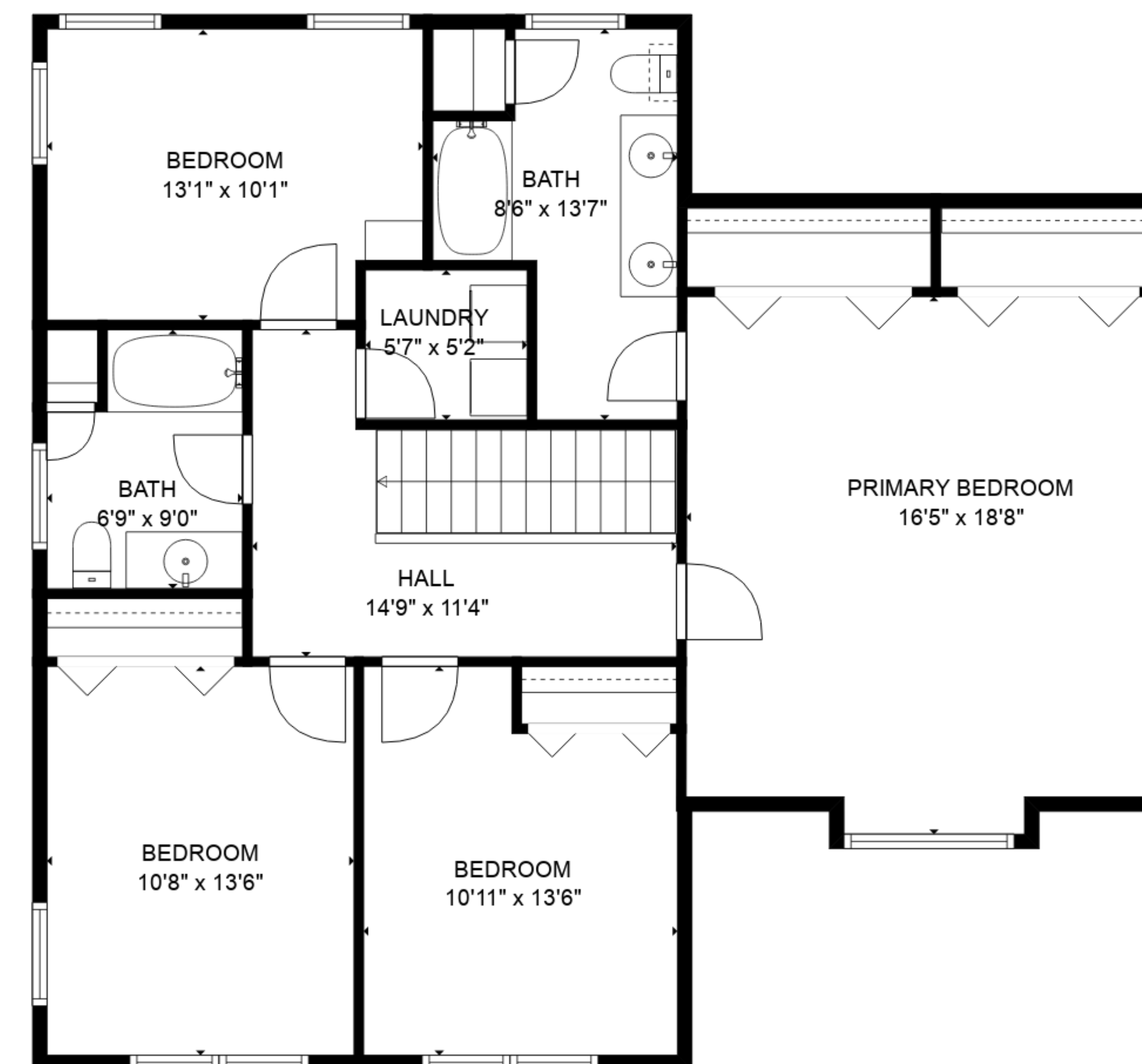
FLOOR 3
