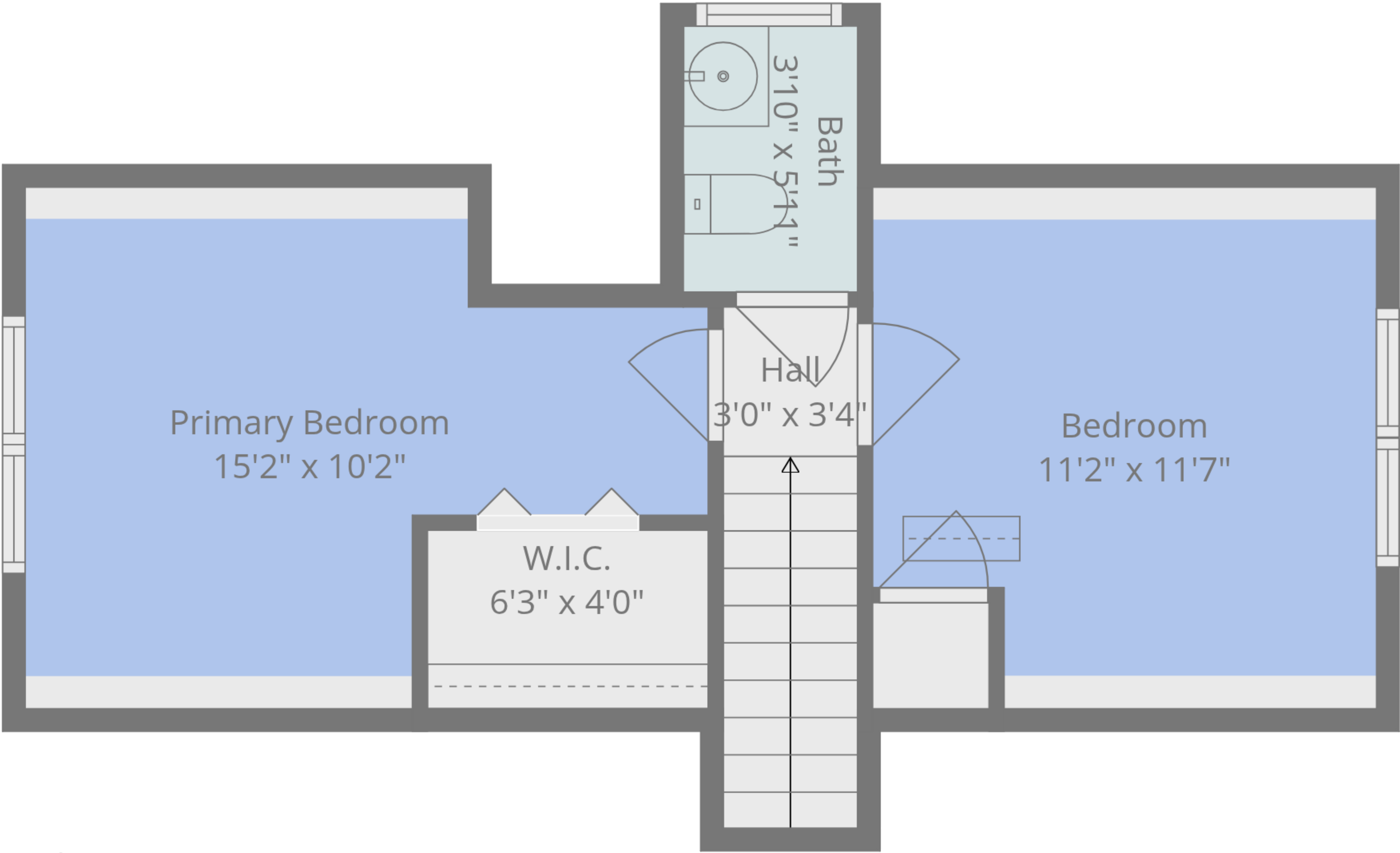
2nd Floor
