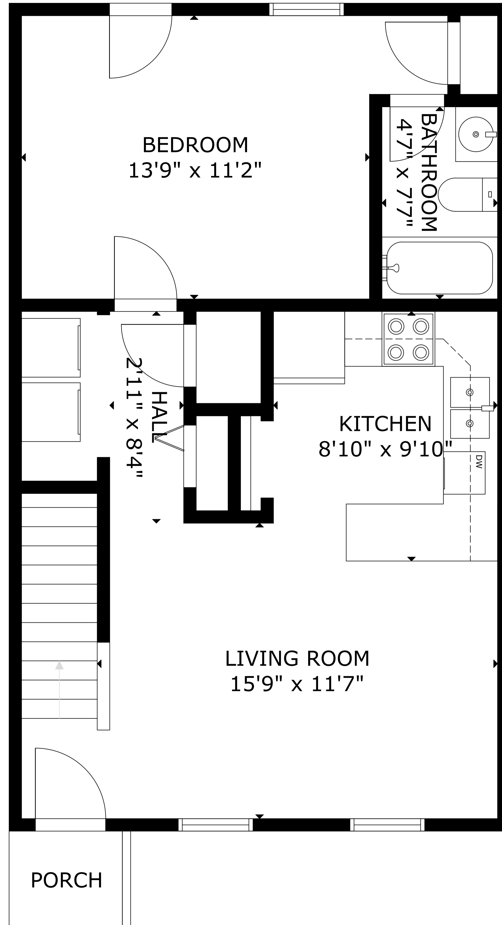
MAIN FLOOR
