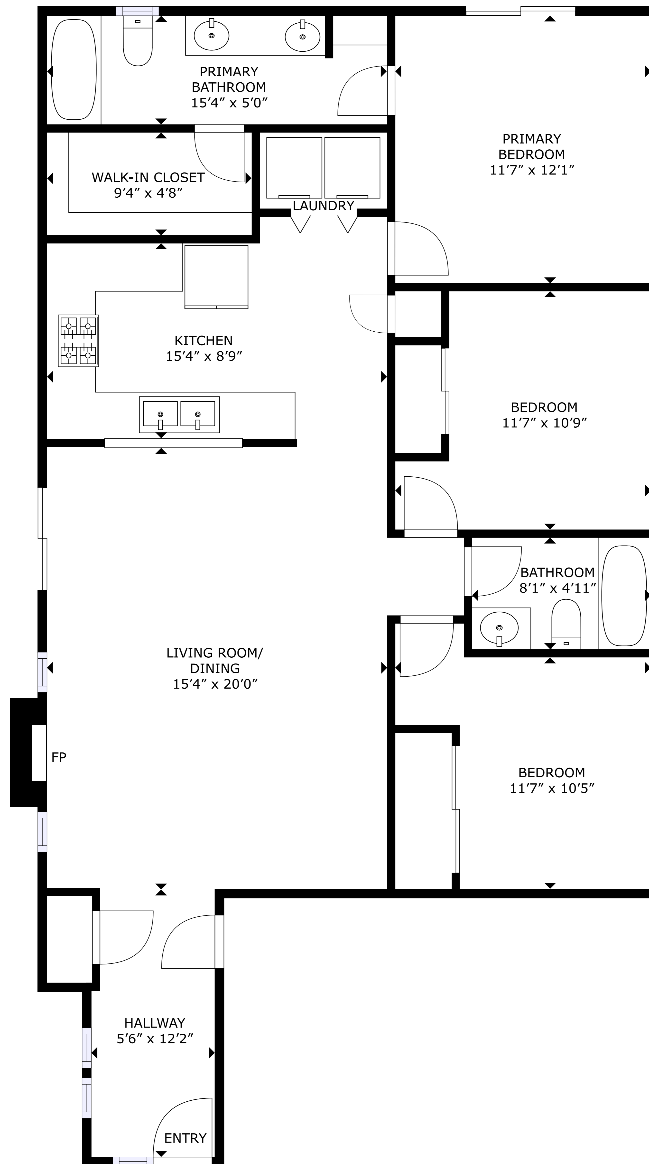
FLOOR PLAN
