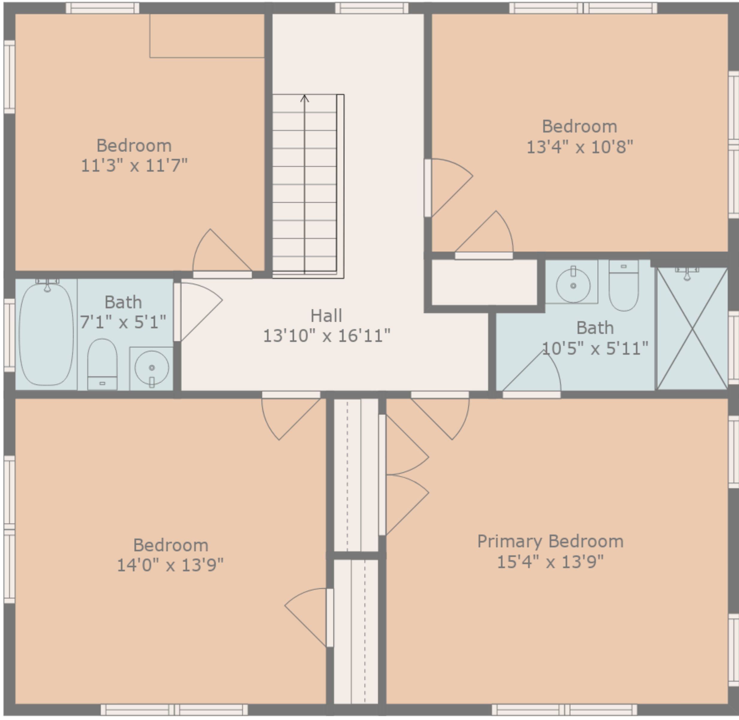
Floor 4
