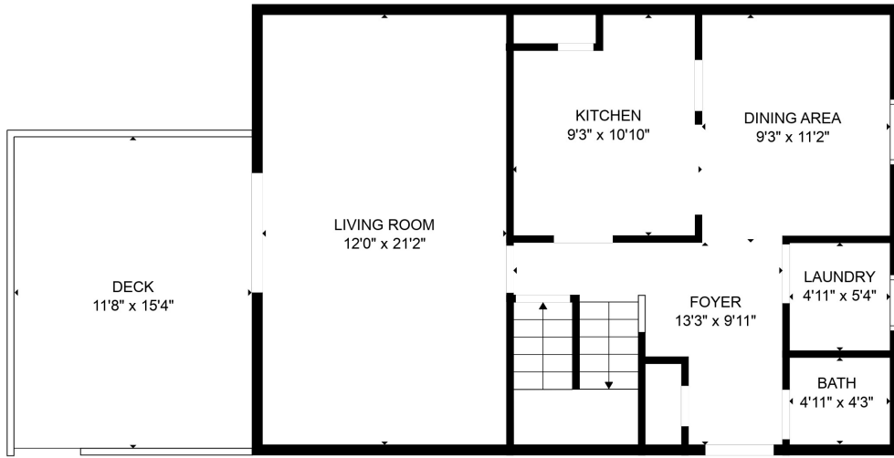
FLOOR 2
