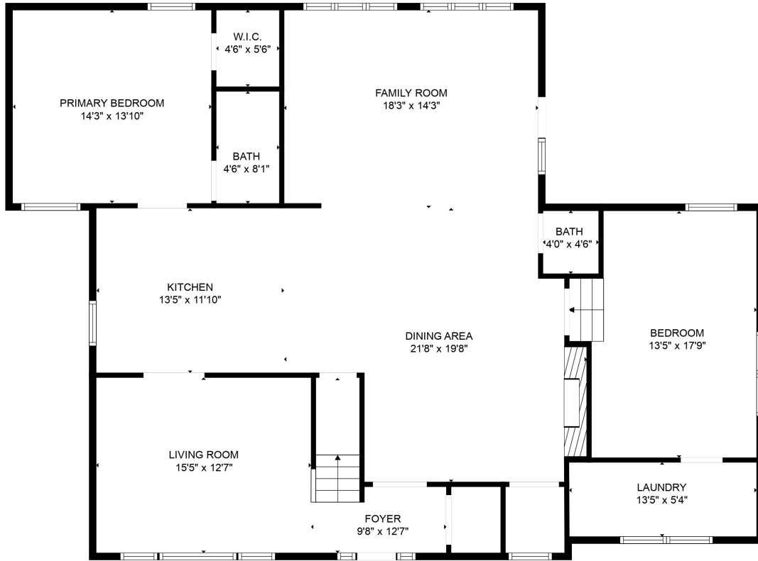
FLOOR 1
