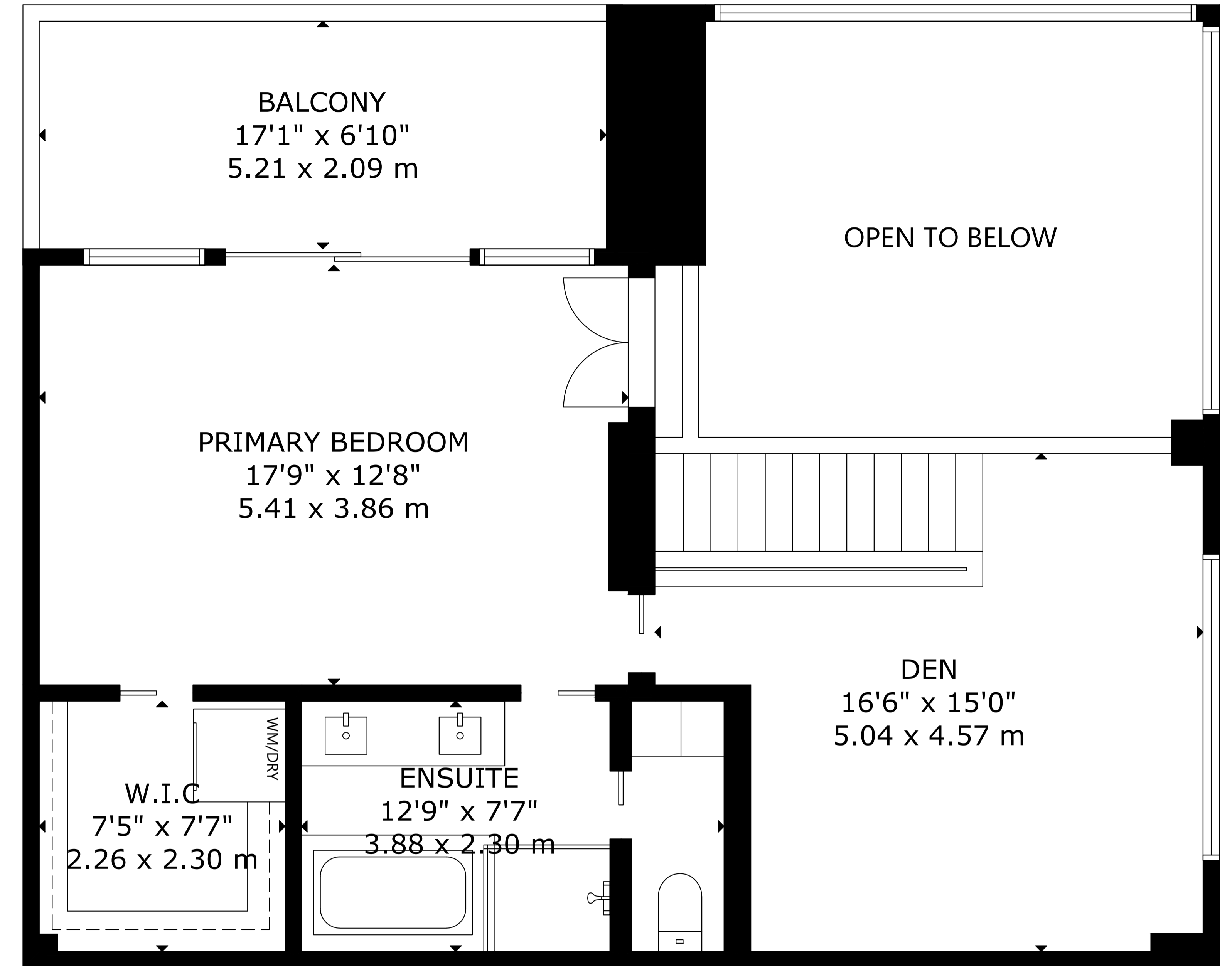
SECOND FLOOR
