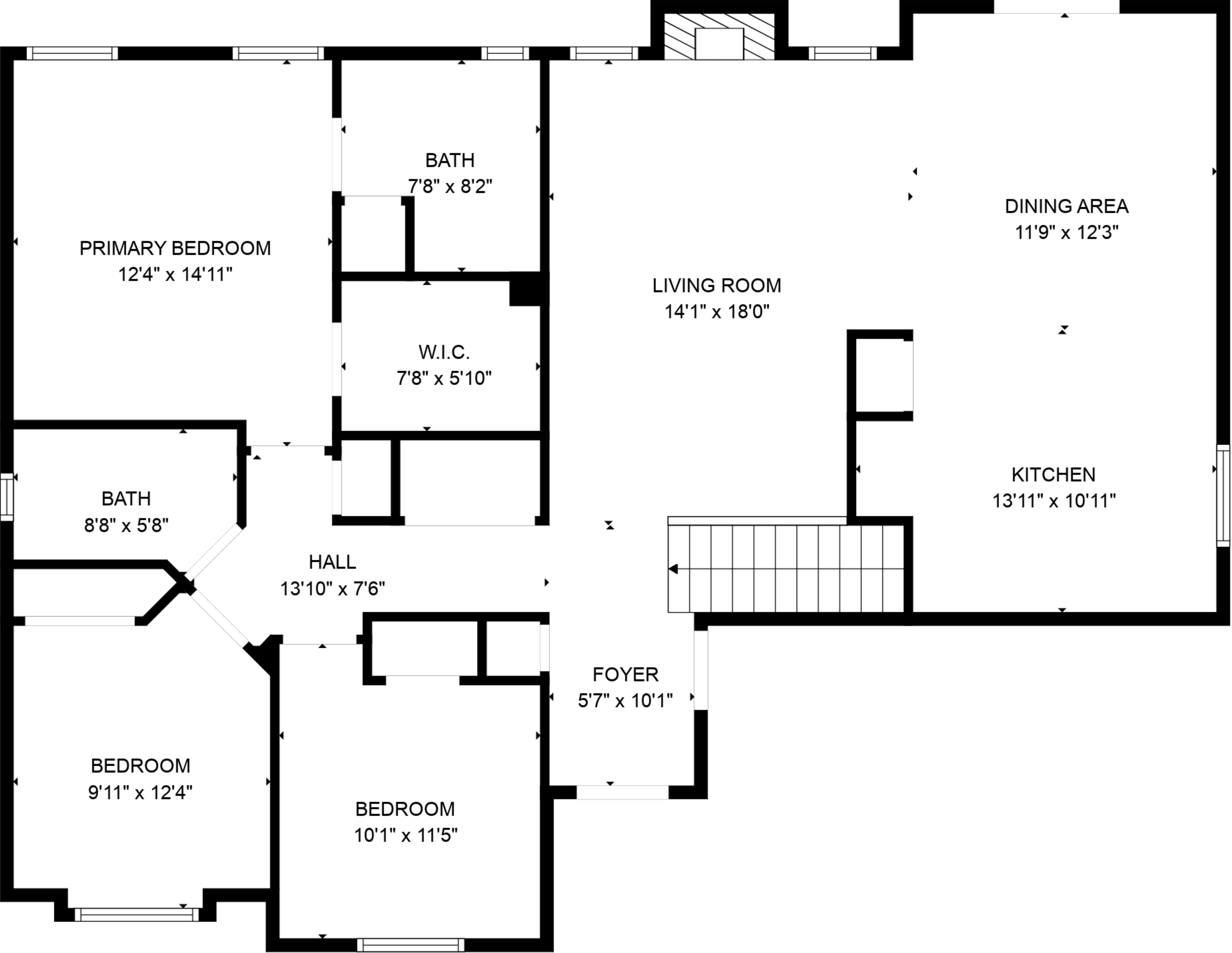
FLOOR 2
