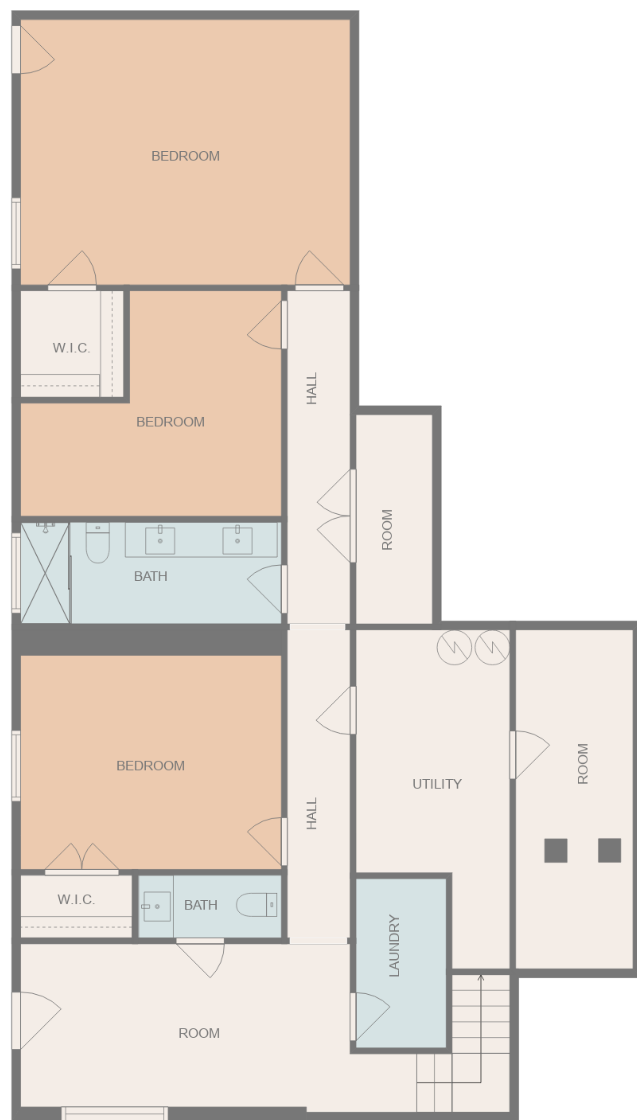
FLOOR 1
