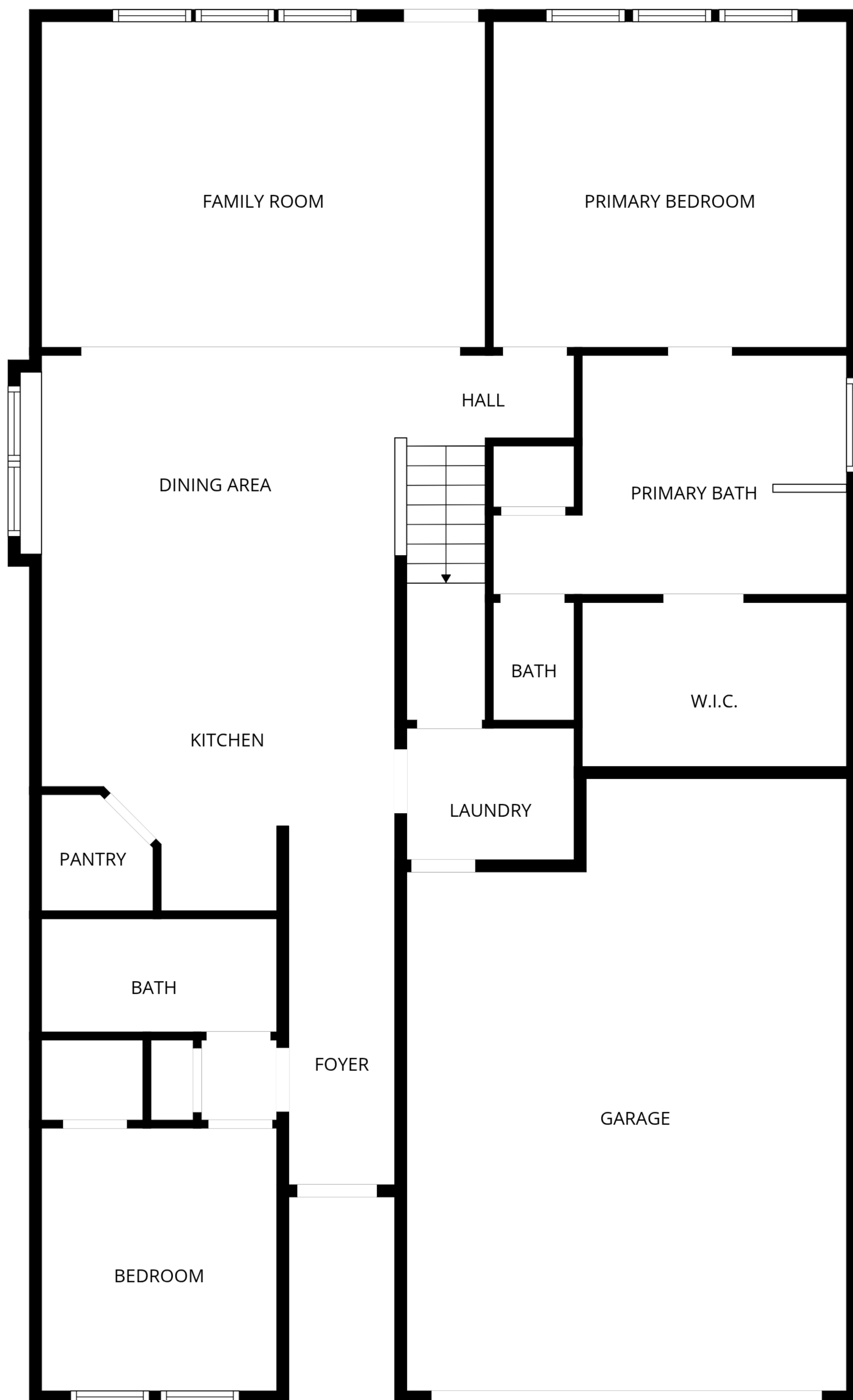
FLOOR 1
