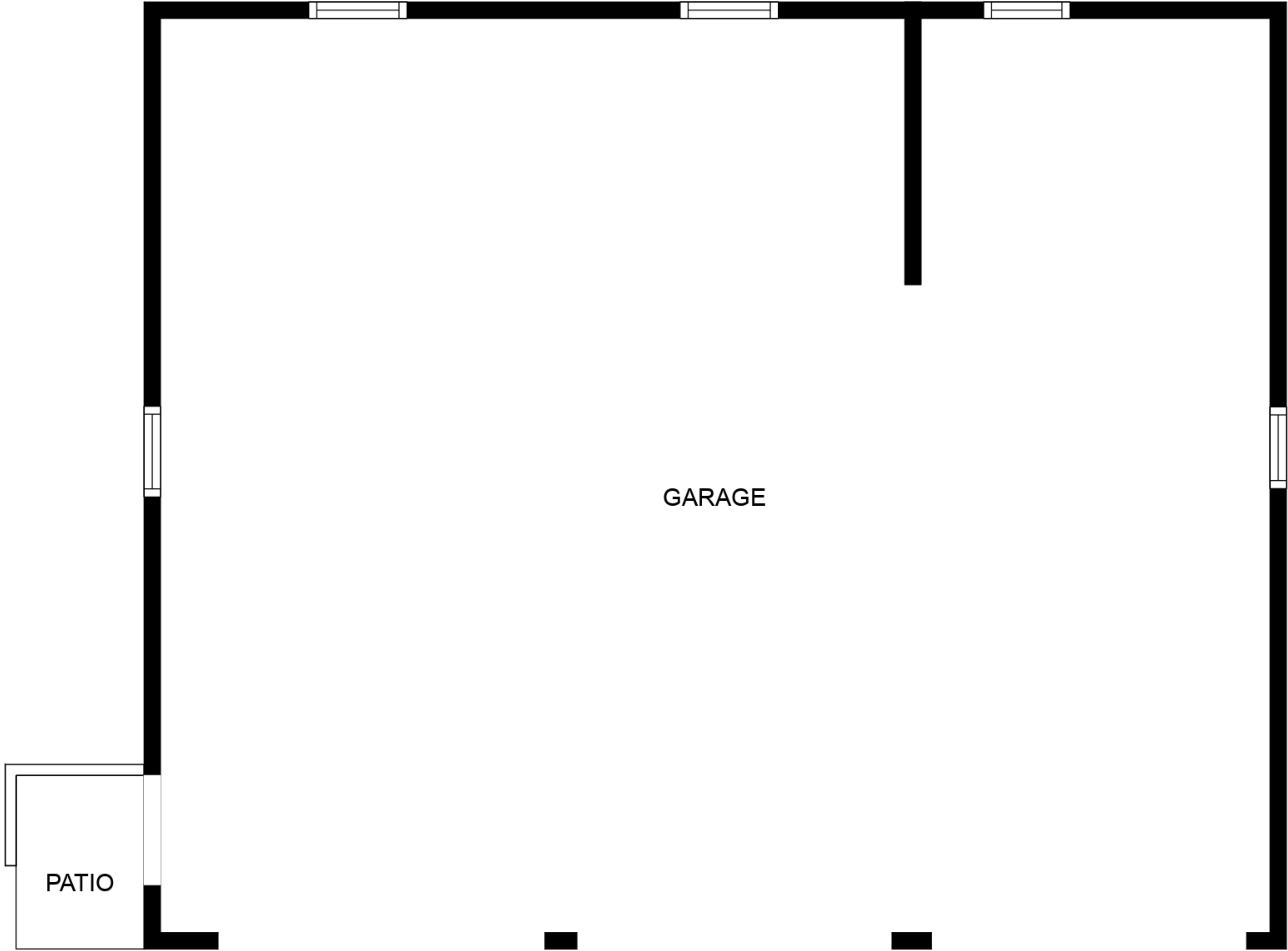
FLOOR 1
