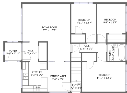
FLOOR 2
