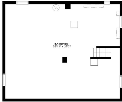
LOWER FLOOR
