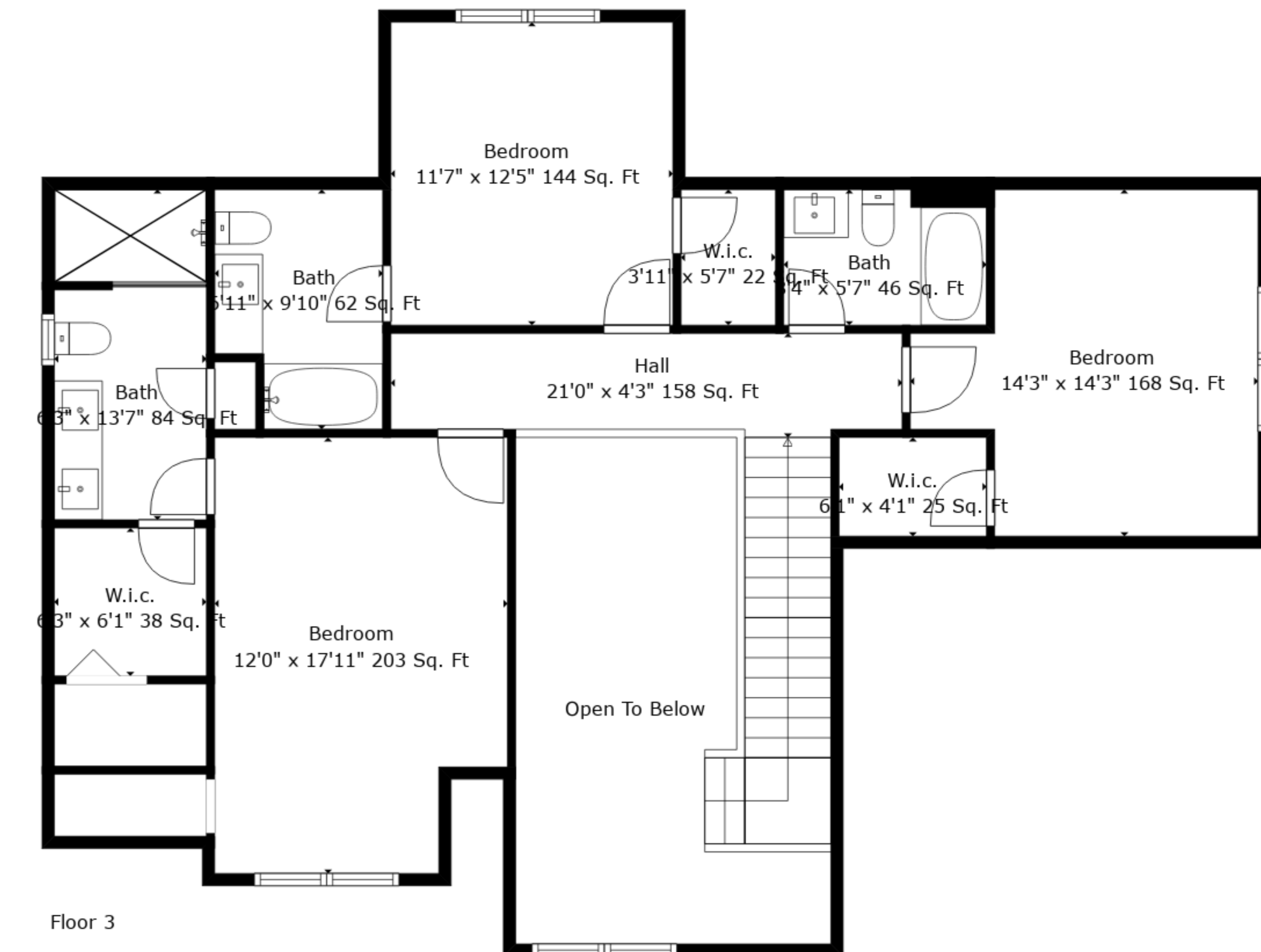
Floor 3
