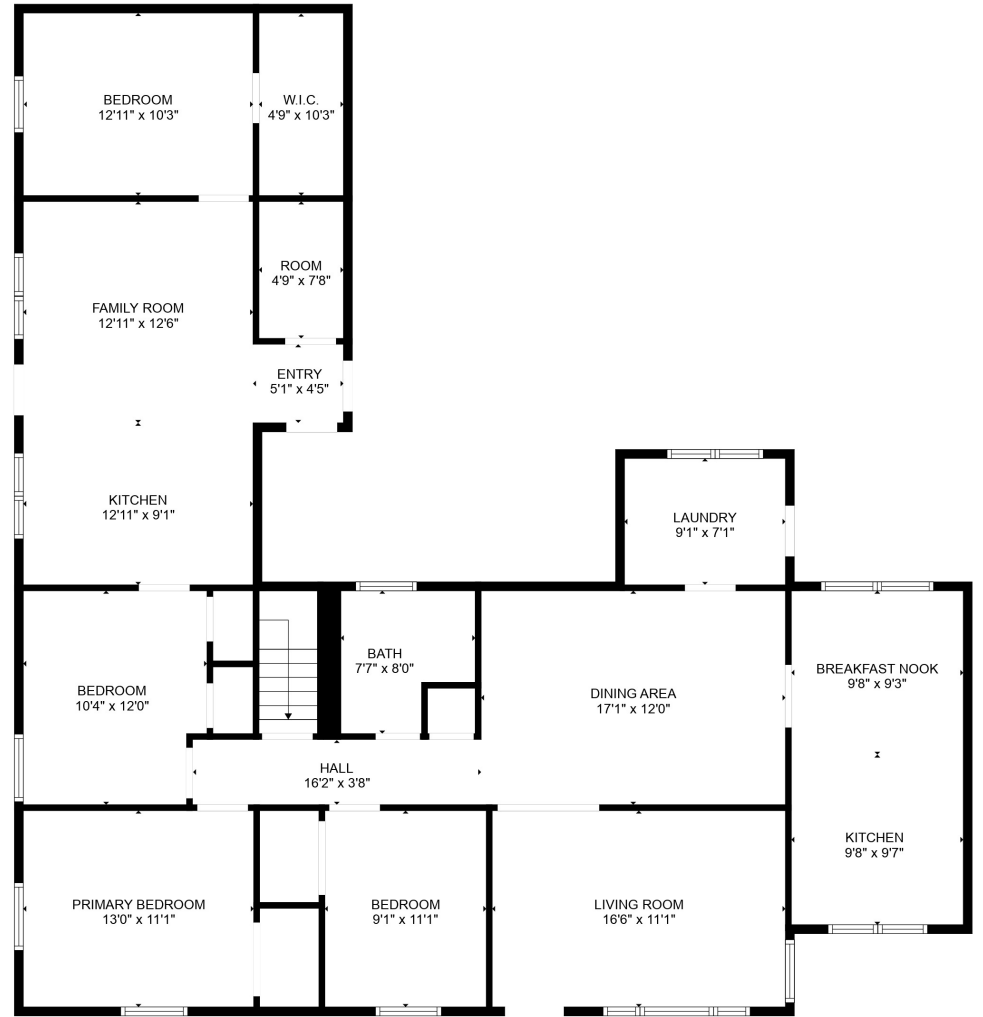
FLOOR 2
