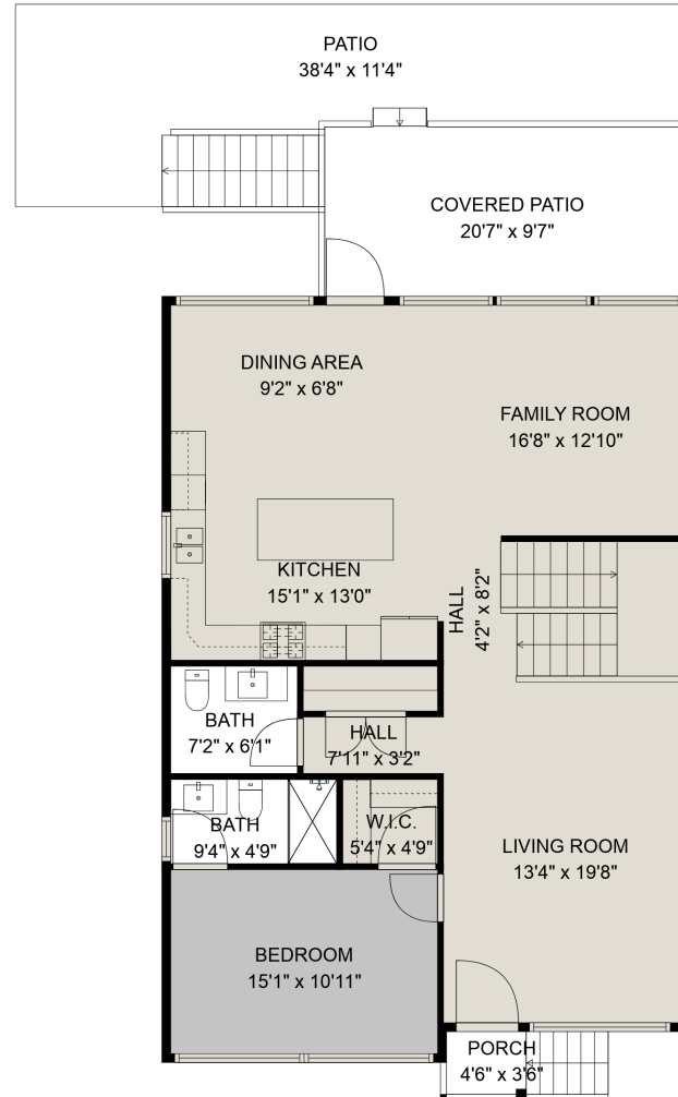
FLOOR 2
